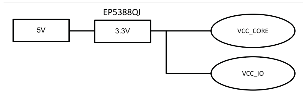
Figure 3-4. Power Distribution System
