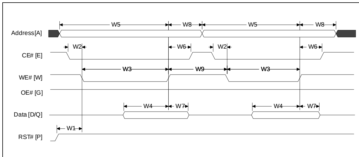
Figure 24: Write-to-Write Timing
