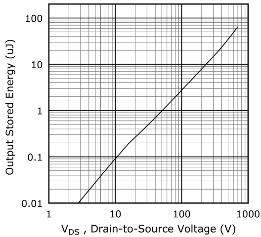
Figure 1-9. Output Stored Energy vs. V_{DS}
