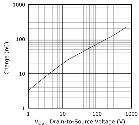
Figure 1-8. Output Charge vs. Drain-to-Source Voltage
