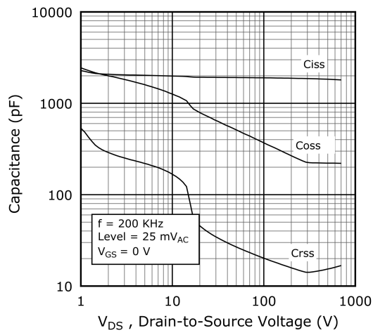
Figure 1-7. Capacitance vs. Drain-to-Source Voltage
