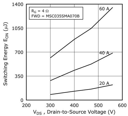
Figure 1-12. Switching Energy E_{on} vs. V_{DS} & I_D
