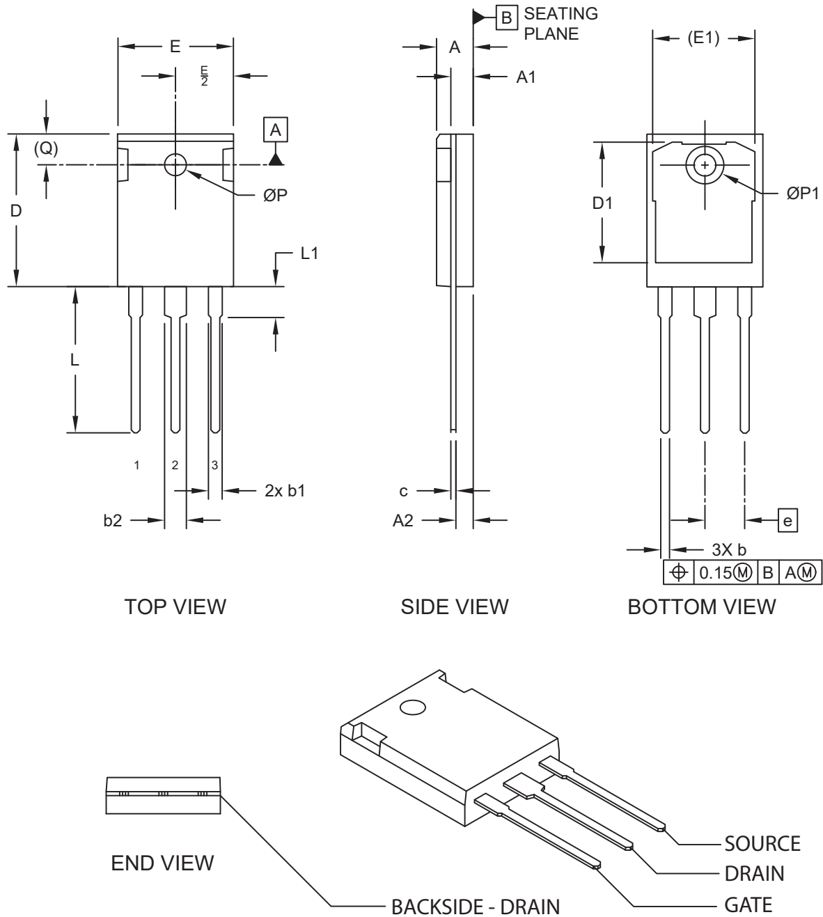
Figure 2-1. Package Outline Drawing
