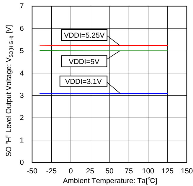
Figure 89. SO "H" Level Output Voltage vs Temperature Characteristic ( I_{SOURCE} = 200\mu A )
