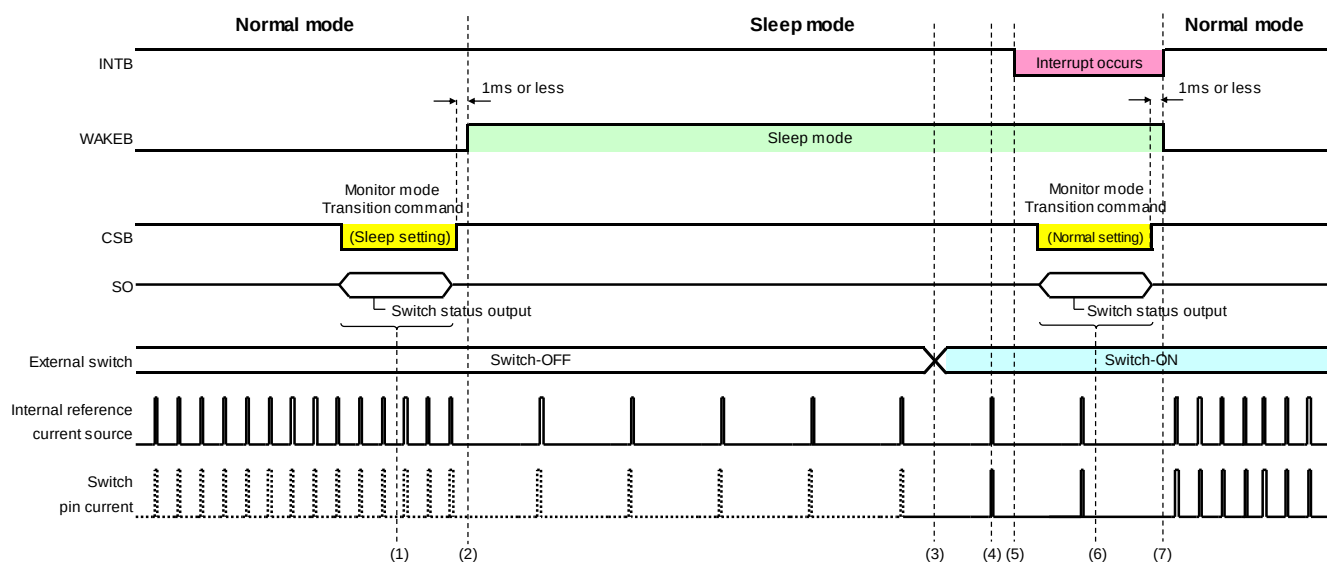
Figure 9. Basic Operation 3
