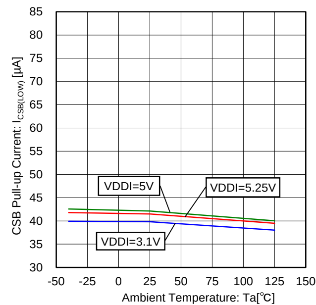
Figure 83. CSB Pull-up Current vs Temperature Characteristic (CSB=0V)
