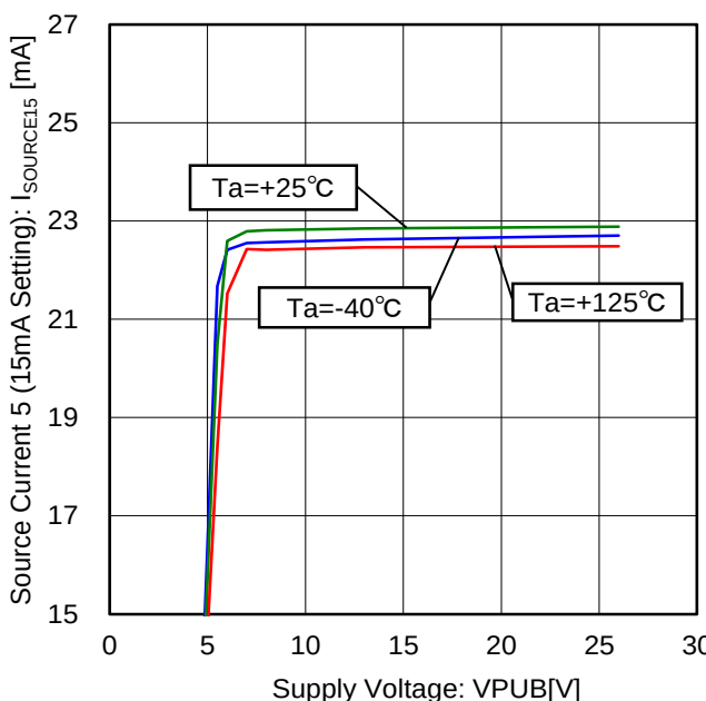
Figure 64. Source Current 5 vs Voltage Characteristic (15mA Setting, 0V external supply)
