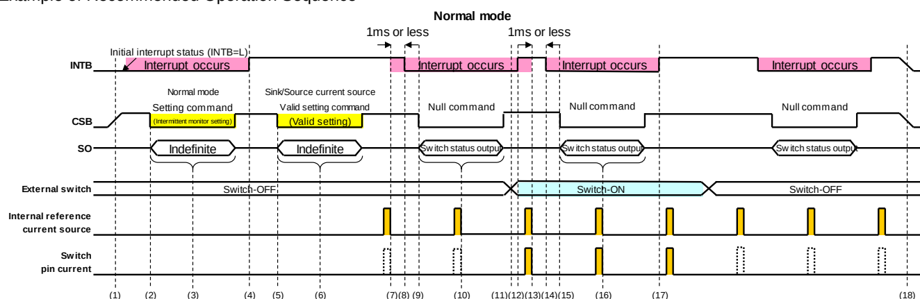
Figure 8. Basic Operation 2
