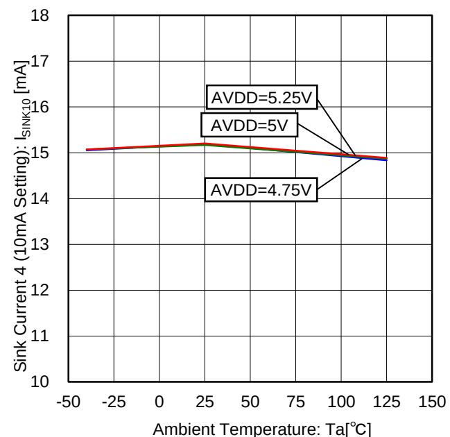
Figure 59. Sink Current 4 vs Temperature Characteristic (10mA Setting, 8V external supply)
