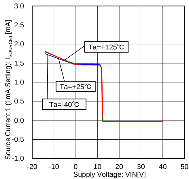
Figure 34. Source Current 1 vs Voltage Characteristic (1mA Setting)
