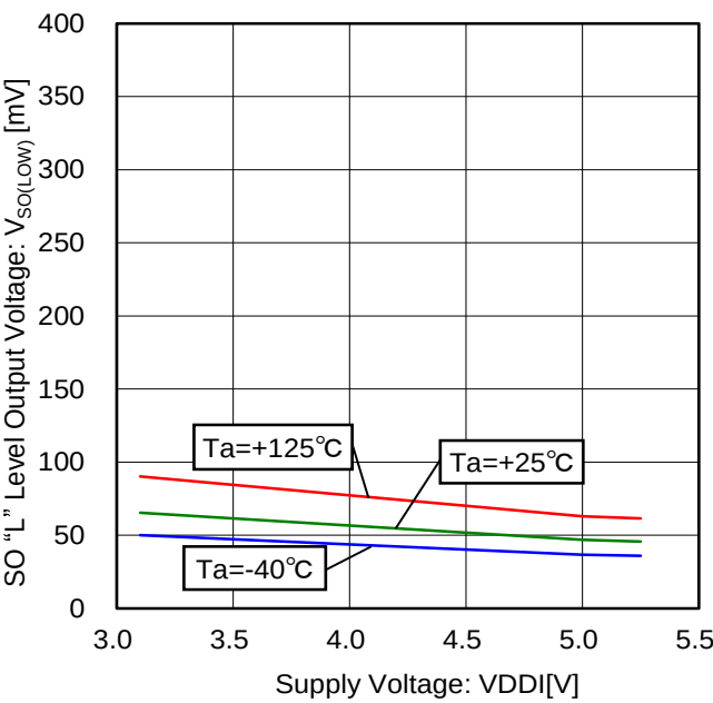
Figure 92. SO "L" Level Output Voltage vs Voltage Characteristic ( I_{SINK} = 1.6mA )
