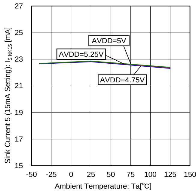
Figure 67. Sink Current 5 vs Temperature Characteristic (15mA Setting, 8V external supply)
