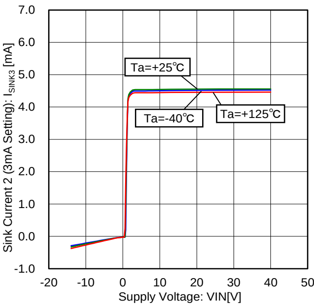
Figure 46. Sink Current 2 vs Voltage Characteristic (3mA Setting)
