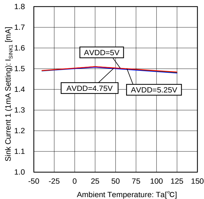
Figure 35. Sink Current 1 vs Temperature Characteristic (1mA Setting, 8V external supply)
