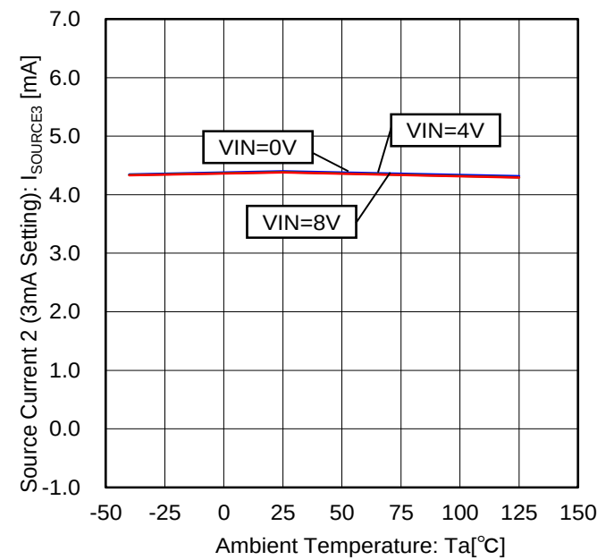
Figure 41. Source Current 2 vs Temperature Characteristic (3mA Setting)
