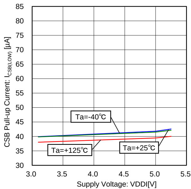
Figure 84. CSB Pull-up Current vs Voltage Characteristic (CSB=0V)
