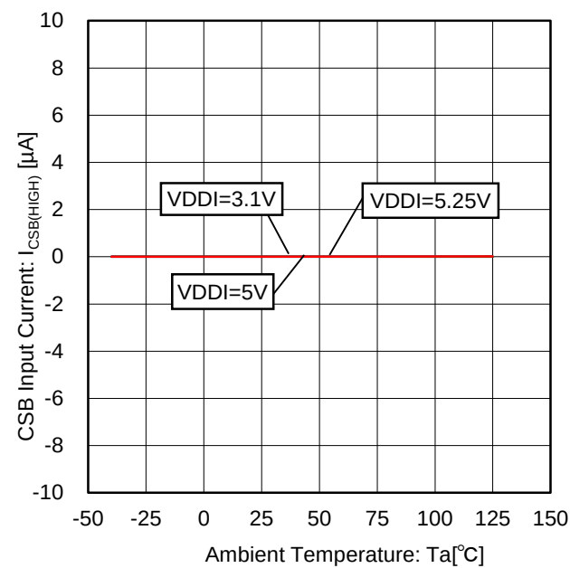
Figure 81. CSB Input Current vs Temperature Characteristic (CSB=VDDI)
