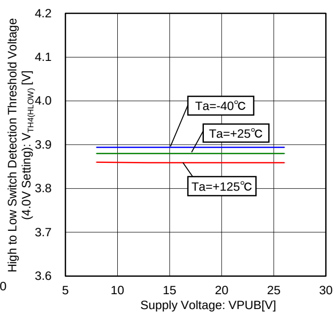
Figure 78. High to Low Switch Detection Threshold Voltage vs Voltage Characteristic (4.0V Setting)
