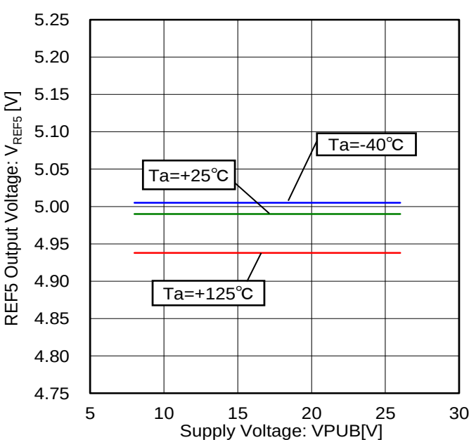
Figure 30. REF5 Output Voltage vs Voltage Characteristic
