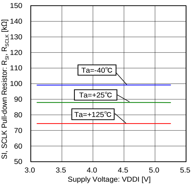
Figure 86. SI, SCLK Pull-down Resistor vs Voltage Characteristic
