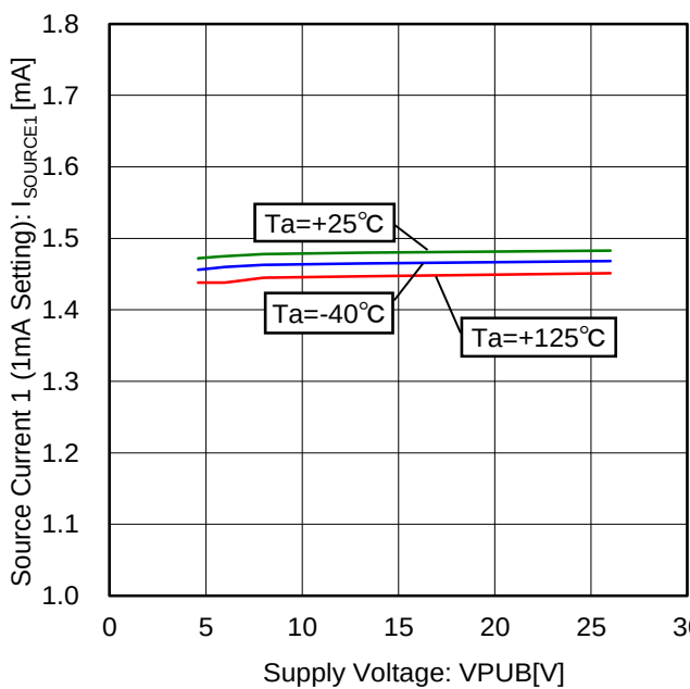
Figure 32. Source Current 1 vs Voltage Characteristic (1mA Setting, 0V external supply)
