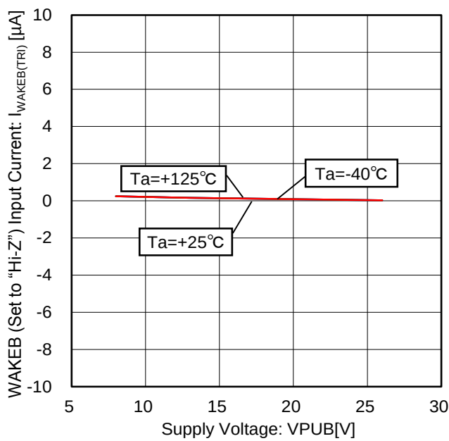
Figure 108. WAKEB (Set to "Hi-Z") Input Current vs Voltage Characteristic
