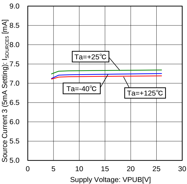
Figure 48. Source Current 3 vs Voltage Characteristic (5mA Setting, 0V external supply)
