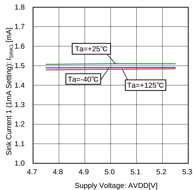
Figure 36. Sink Current 1 vs Voltage Characteristic (1mA Setting, 8V external supply)
