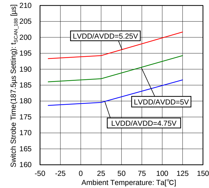
Figure 113. Switch Strobe Time vs Temperature Characteristic (187.5µs Setting)
