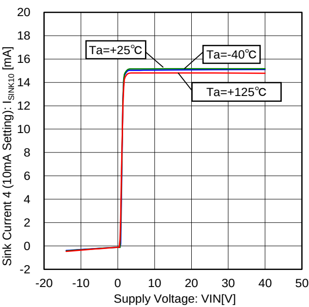
Figure 62. Sink Current 4 vs Voltage Characteristic (10mA Setting)
