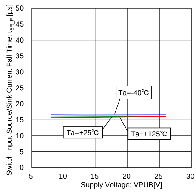
Figure 120. Switch Input Source/Sink Current Fall Time vs Voltage Characteristic (FSQ="0", FSQZ/A/B="0", 10mA Setting, Load Resistance=100Ω)
