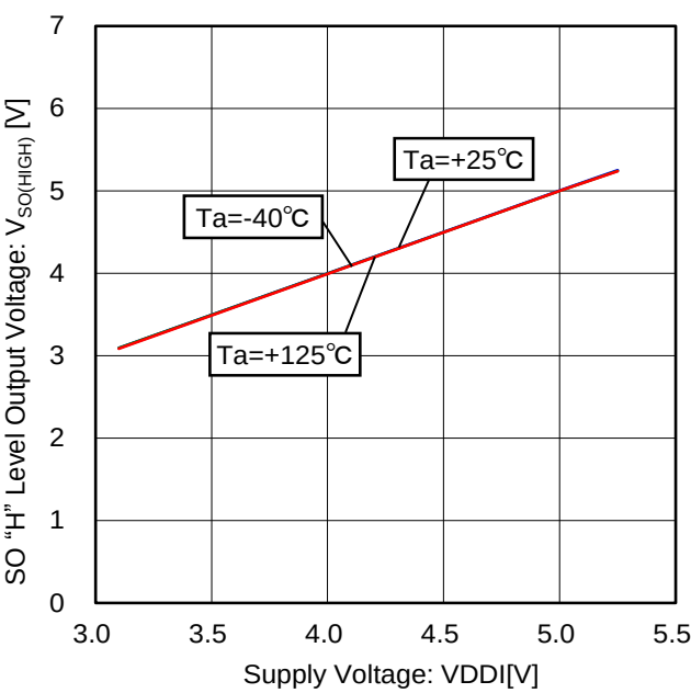
Figure 90. SO "H" Level Output Voltage vs Voltage Characteristic ( I_{SOURCE} = 200\mu A )
