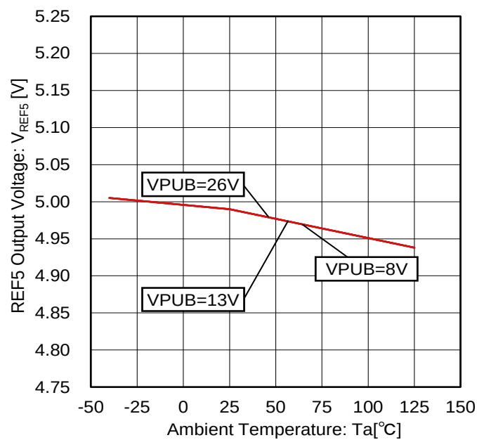
Figure 29. REF5 Output Voltage vs Temperature Characteristic
