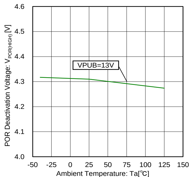
Figure 22. POR (Power on Reset) Deactivation Voltage vs Temperature Characteristic
