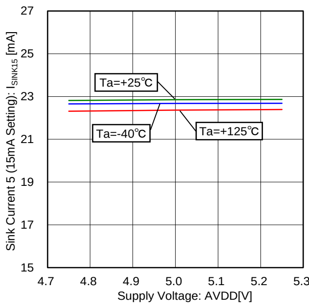
Figure 68. Sink Current 5 vs Voltage Characteristic (15mA Setting, 8V external supply)
