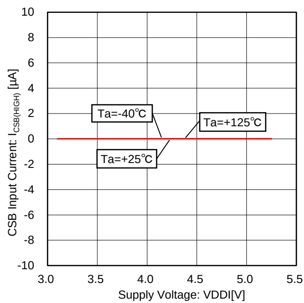
Figure 82. CSB Input Current vs Voltage Characteristic (CSB=VDDI)
