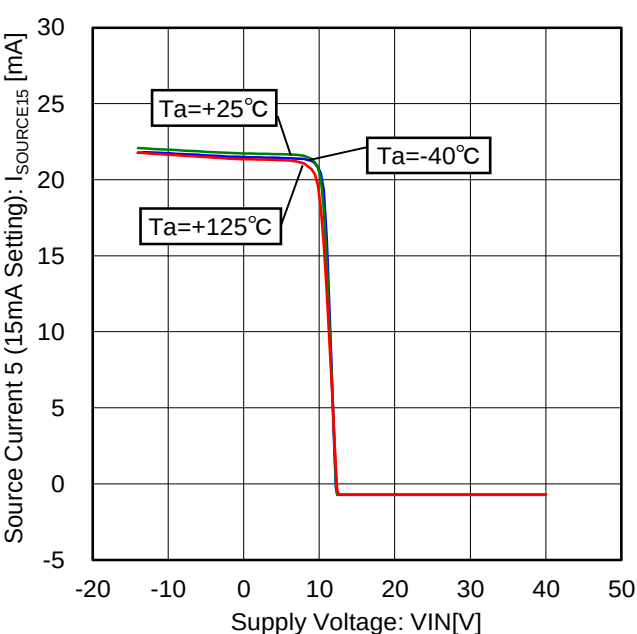
Figure 66. Source Current 5 vs Voltage Characteristic (15mA Setting)
