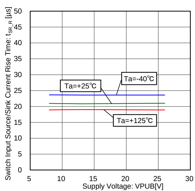
Figure 118. Switch Input Source/Sink Current Rise Time vs Voltage Characteristic (FSQ="0", FSQZ/A/B="0", 10mA Setting, Load Resistance=100Ω)
