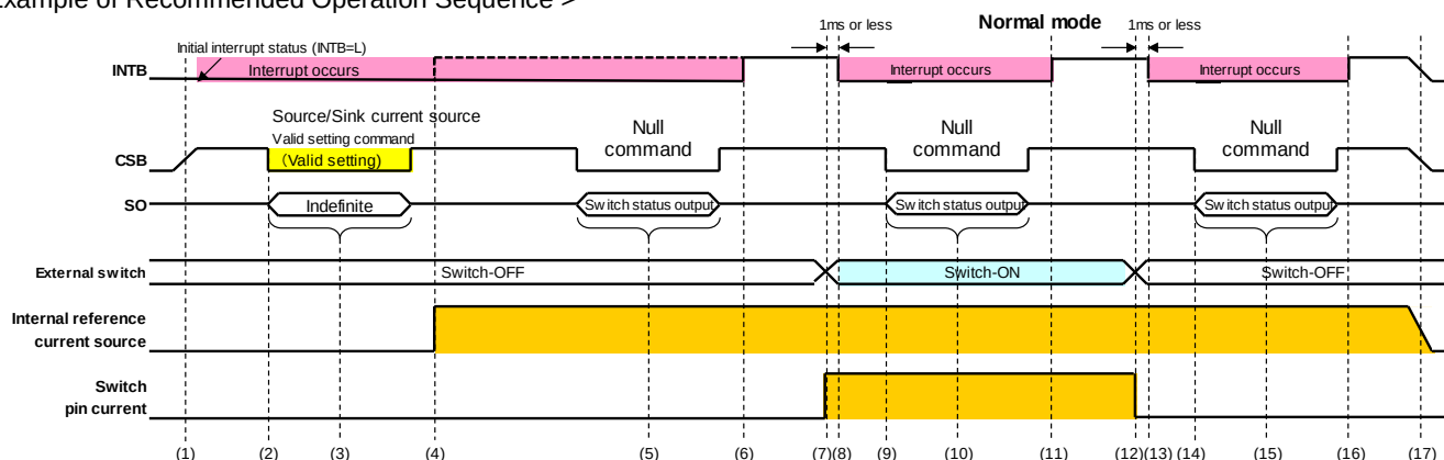
Figure 7. Basic Operation 1
