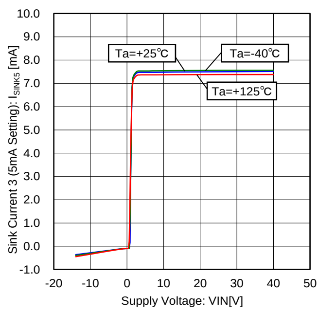
Figure 54. Sink Current 3 vs Voltage Characteristic (5mA Setting)
