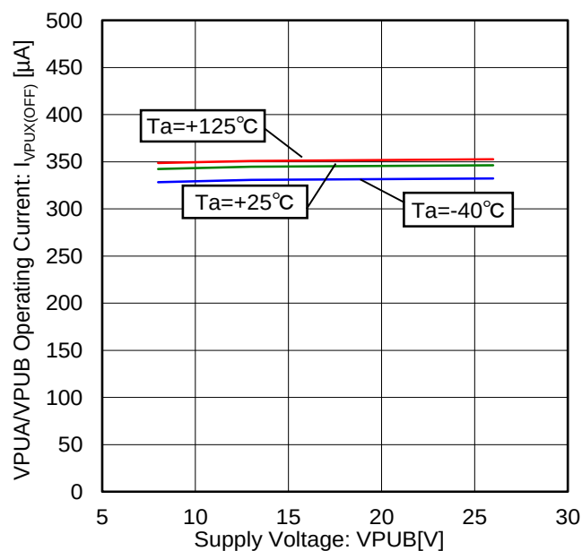
Figure 24. VPUA/VPUB Operating Current vs Voltage Characteristic (Continuous monitor setting, Current source is invalid, "Hi-Z" Status)
