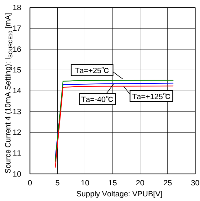
Figure 56. Source Current 4 vs Voltage Characteristic (10mA Setting, 0V external supply)
