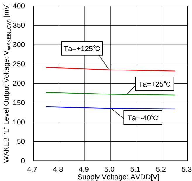
Figure 106. WAKEB "L" Level Output Voltage vs Voltage Characteristic (WAKEB=1.0mA)
