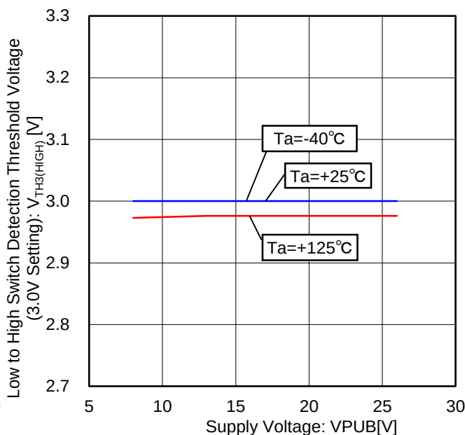
Figure 72. Low to High Switch Detection Threshold Voltage vs Voltage Characteristic (3.0V Setting)
