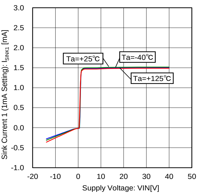
Figure 38. Sink Current 1 vs Voltage Characteristic (1mA Setting)
