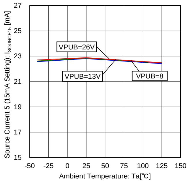
Figure 63. Source Current 5 vs Temperature Characteristic (15mA Setting, 0V external supply)
