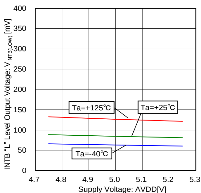
Figure 104. INTB "L" Level Output Voltage vs Voltage Characteristic ( I_{SINK} = 1.0mA )
