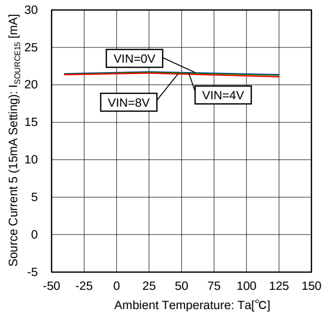
Figure 65. Source Current 5 vs Temperature Characteristic (15mA Setting)
