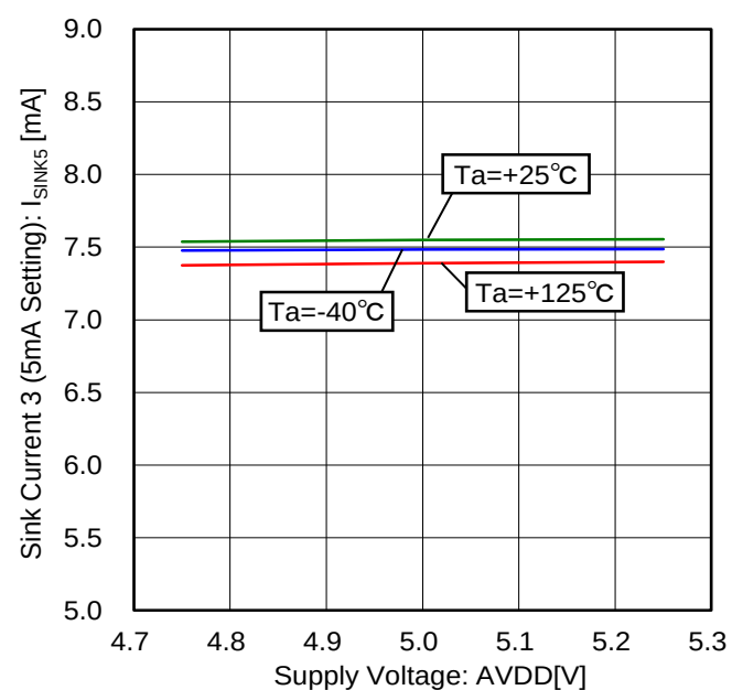
Figure 52. Sink Current 3 vs Voltage Characteristic (5mA Setting, 8V external supply)
