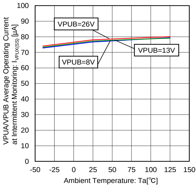
Figure 25. VPUA/VPUB Average Operating Current at Intermittent Monitoring vs Temperature Characteristic (Monitoring Period: 50ms, Strobe Time: 125 \mu s , Source/Sink Current Setting: 1mA)
