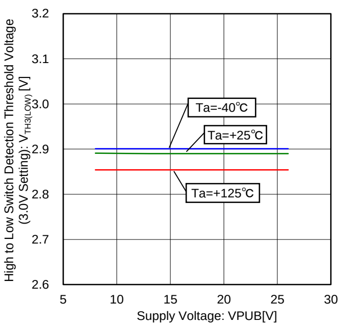
Figure 74. High to Low Switch Detection Threshold Voltage vs Voltage Characteristic (3.0V Setting)
