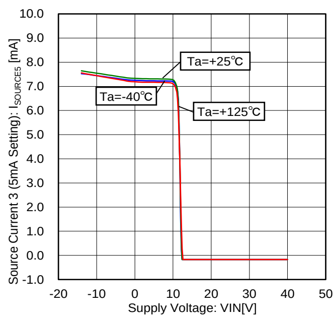
Figure 50. Source Current 3 vs Voltage Characteristic (5mA Setting)
