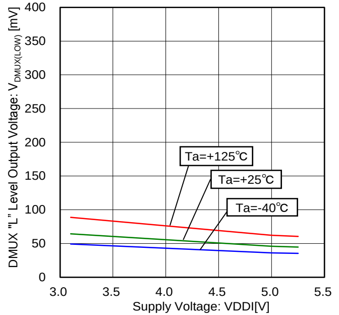
Figure 98. DMUX "L" Level Output Voltage vs Voltage Characteristic ( I_{SINK}=1.6mA )
