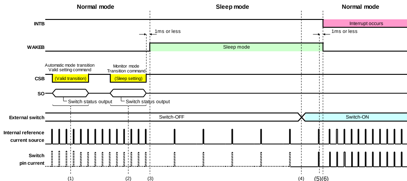
Figure 10. Basic Operation 4
