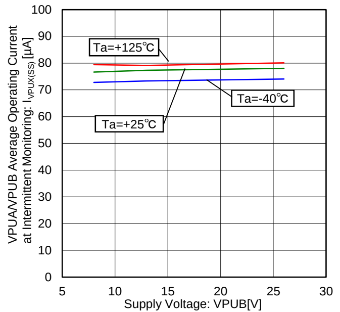
Figure 26. VPUA/VPUB Average Operating Current at Intermittent Monitoring vs Voltage Characteristic (Monitoring Period: 50ms, Strobe Time: 125 \mu s , Source/Sink Current Setting: 1mA)
