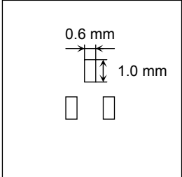
Figure 1: 25.4 mm × 25.4 mm × 1.6 t, Cu Pad: 0.6 mm 2 × 3
