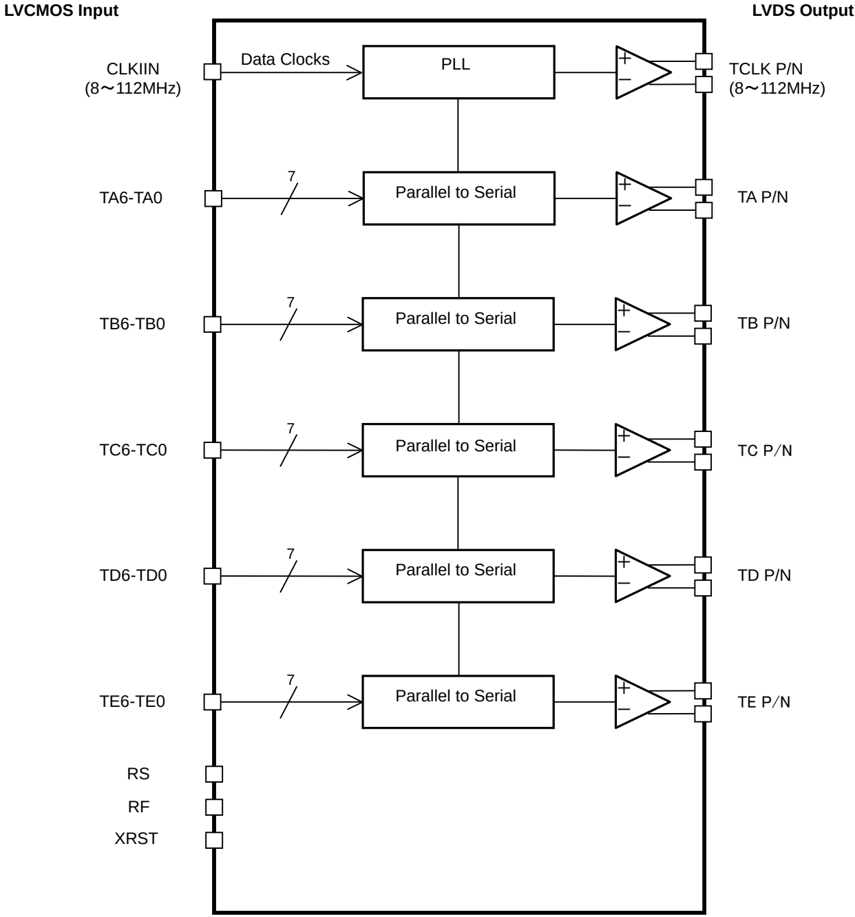
Fig.1 Block Diagram
