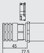
Powerkontakt Stift Contact for power male
