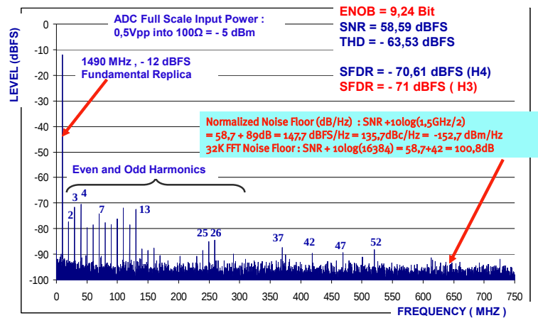
Figure 6-9. FFT 1.5 GSps Fin = 1490 MHz@-12 dBFS
