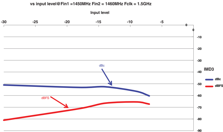
Figure 6-28. IMD3 Vs Input level @ 1.5 GSps Fin1 = 1450 MHz Fin2 = 1460 MHz
