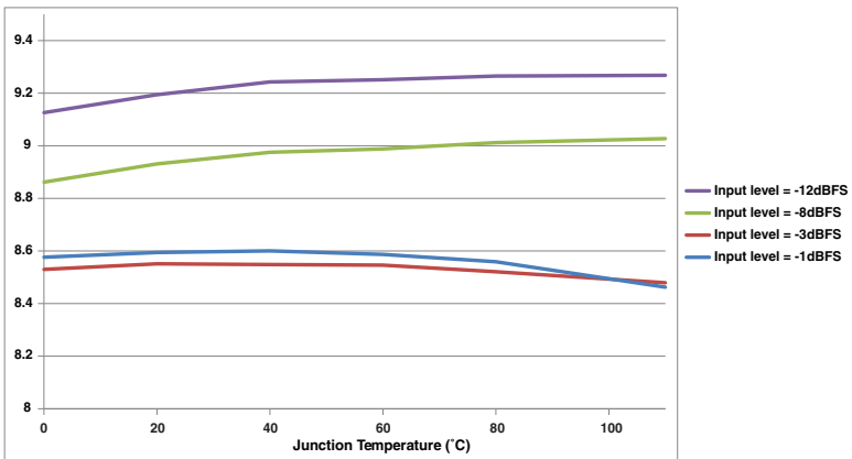
Figure 6-22. ENOB_FS versus Junction Temperature (°C) and Input level @Fin = 1490 MHz
