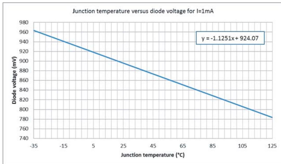
Figure 4-7. Diode characteristics for die junction monitoring
