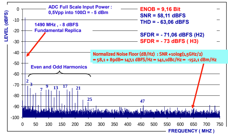
Figure 6-8. FFT 1.5 GSps Fin = 1490 MHz@-8 dBFS
