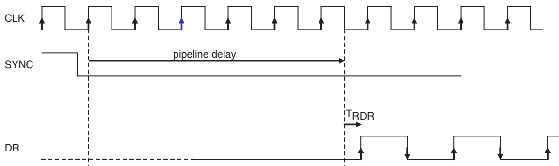
Figure 2-4. SYNC Timing Diagram (1:2 DMUX & Reset Edge: Falling)
