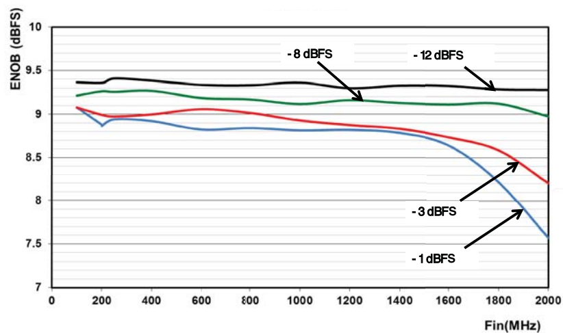
Figure 6-1. ENOB vs Fin from 100 MHz to 2000 MHz@1.5 GSps
