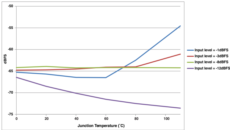
Figure 6-21. SFDR_FS versus Junction Temperature (°C) and Input level @Fin = 740 MHz
