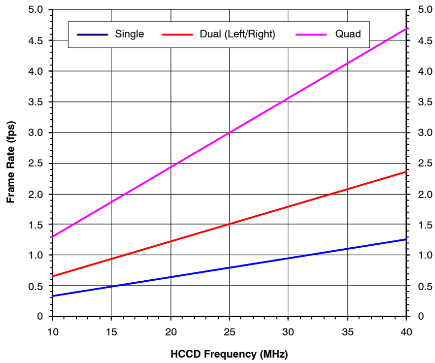
Figure 12. Frame Rates
