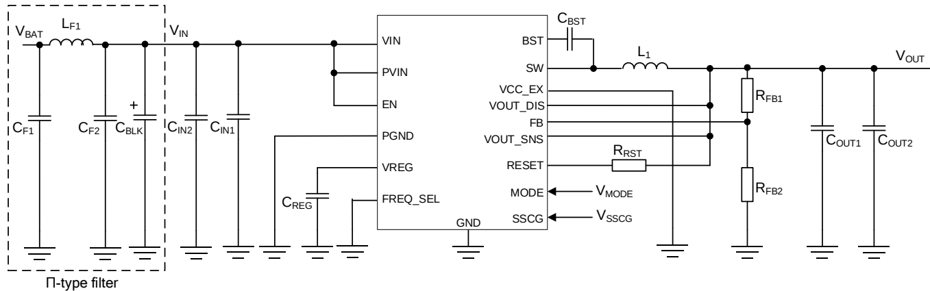
Figure 41. Reference Circuit 1
