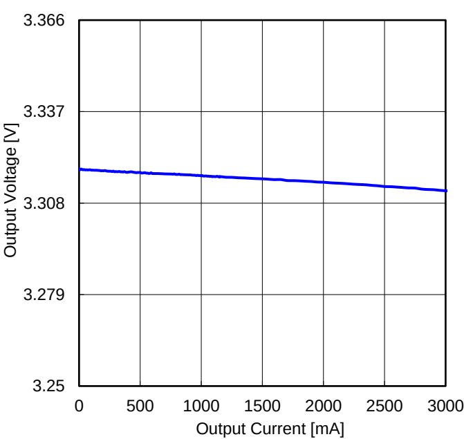
Figure 53. Load Regulation (V IN = 12 V)
