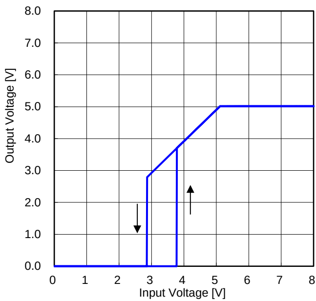
Figure 76. Output Voltage vs Input Voltage 1 ( R_{LOAD} = 166\ \Omega )
