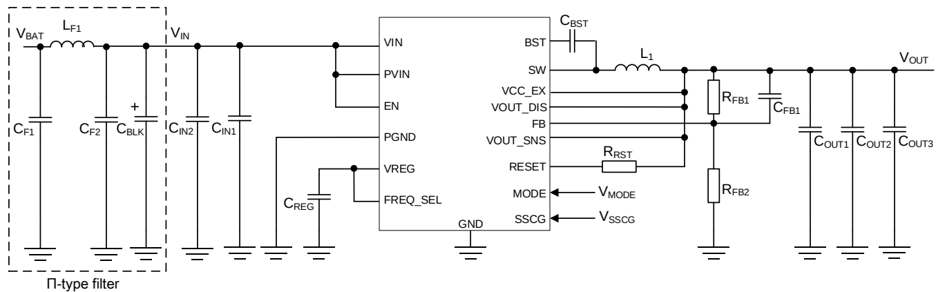
Figure 80. Reference Circuit 4
