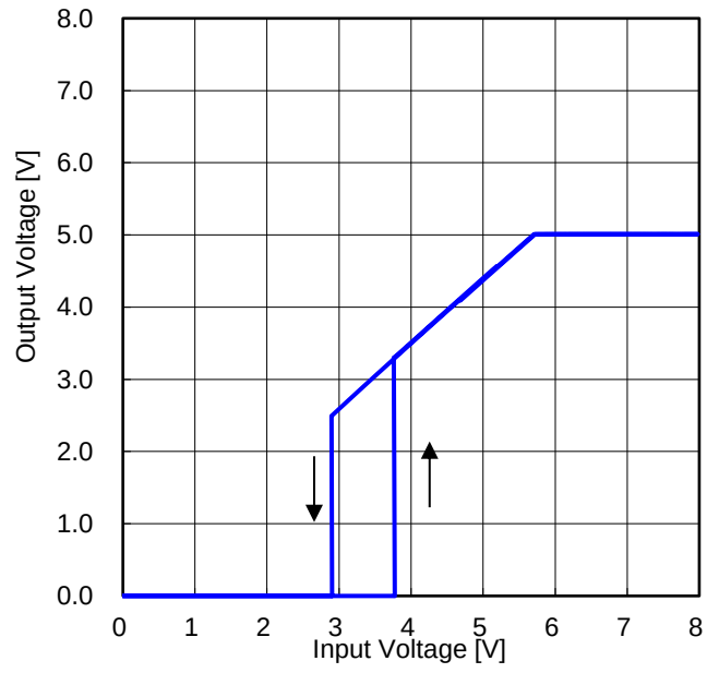
Figure 77. Output Voltage vs Input Voltage 2 ( R_{LOAD} = 1.66\ \Omega )
