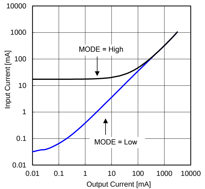
Figure 43. Input Current vs Output Current ( V_{IN} = 12\text{ V} )
