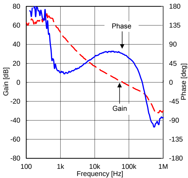
Figure 44. Frequency Characteristic ( V_{IN} = 12\text{ V} , I_{OUT} = 1.5\text{ A} )
