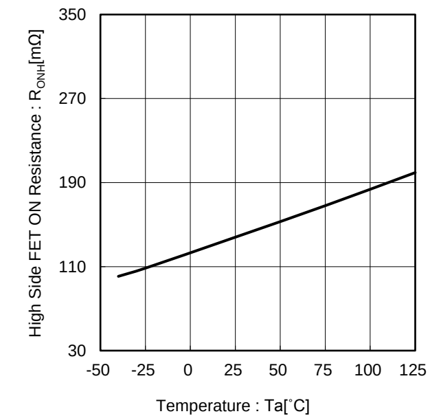
Figure 15. High Side FET ON Resistance vs Temperature
