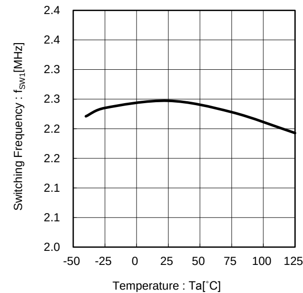
Figure 13. Switching Frequency vs Temperature (FREQ_SEL = Low)
