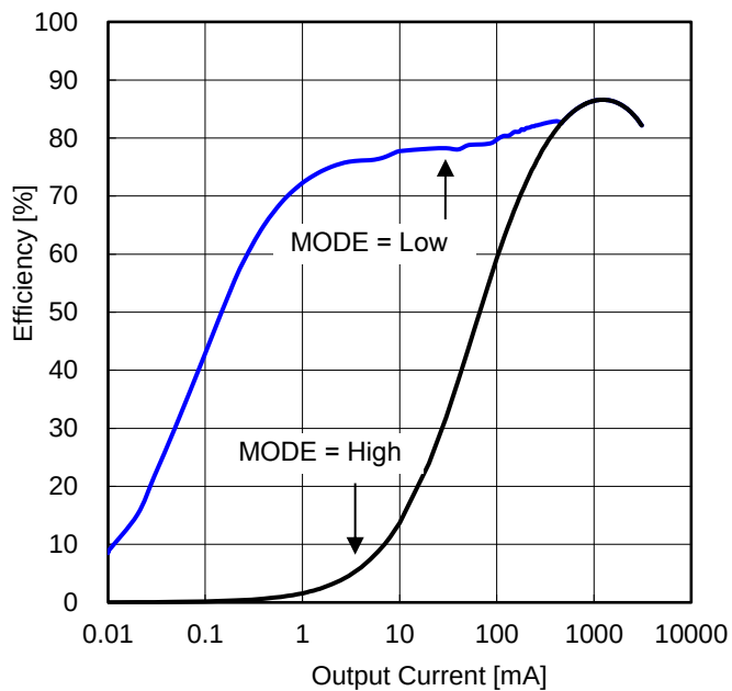
Figure 42. Efficiency vs Output Current ( V_{IN} = 12\text{ V} )
