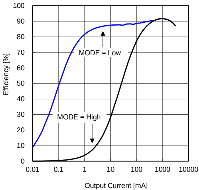
Figure 68. Efficiency vs Output Current ( V_{IN} = 12\text{ V} )
