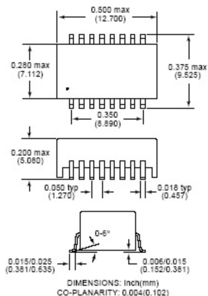
SMD Package
