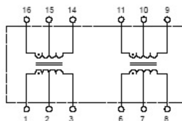
Schematic A
