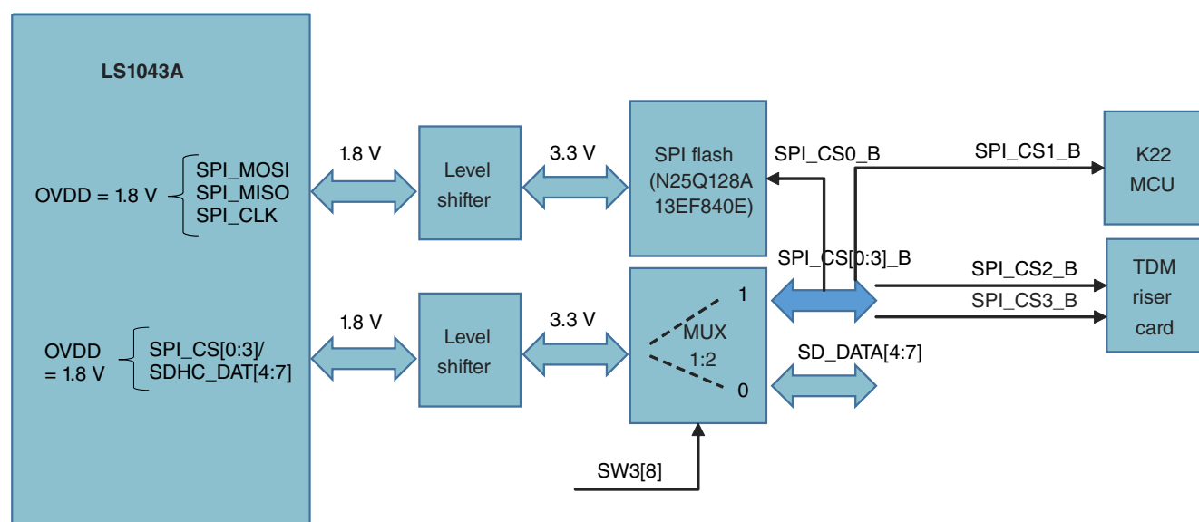
Figure 2-5. DSPI connections
