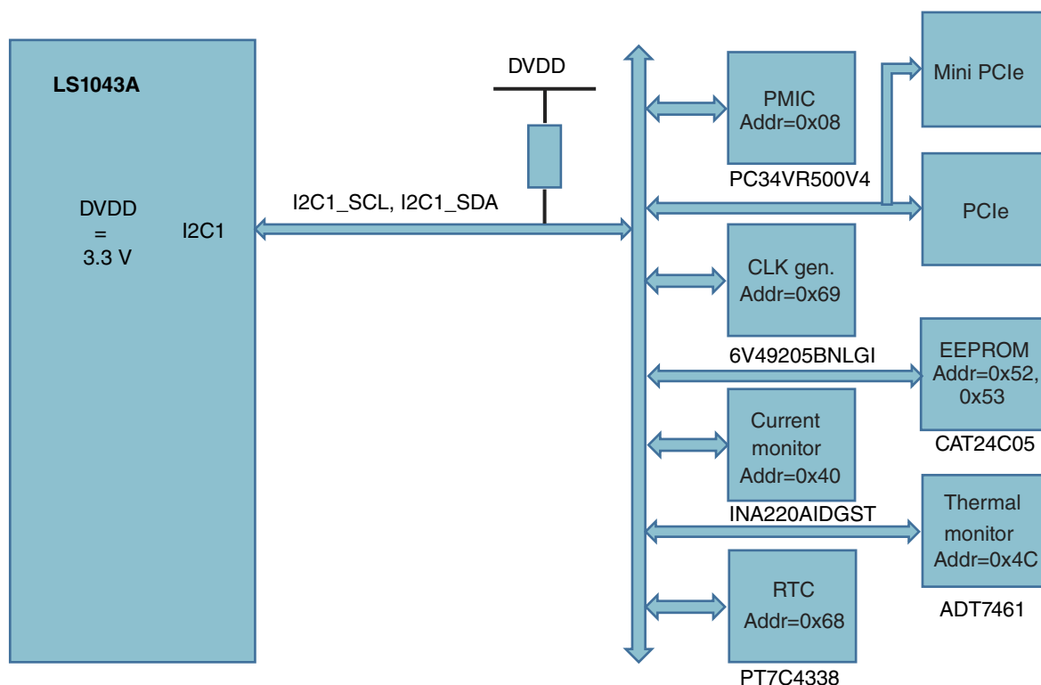
Figure 2-10. I2C scheme
