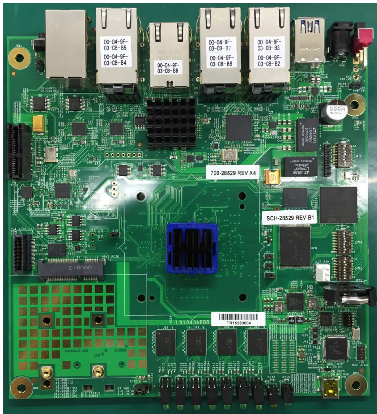
Figure 1-3. LS1043ARDB top view
