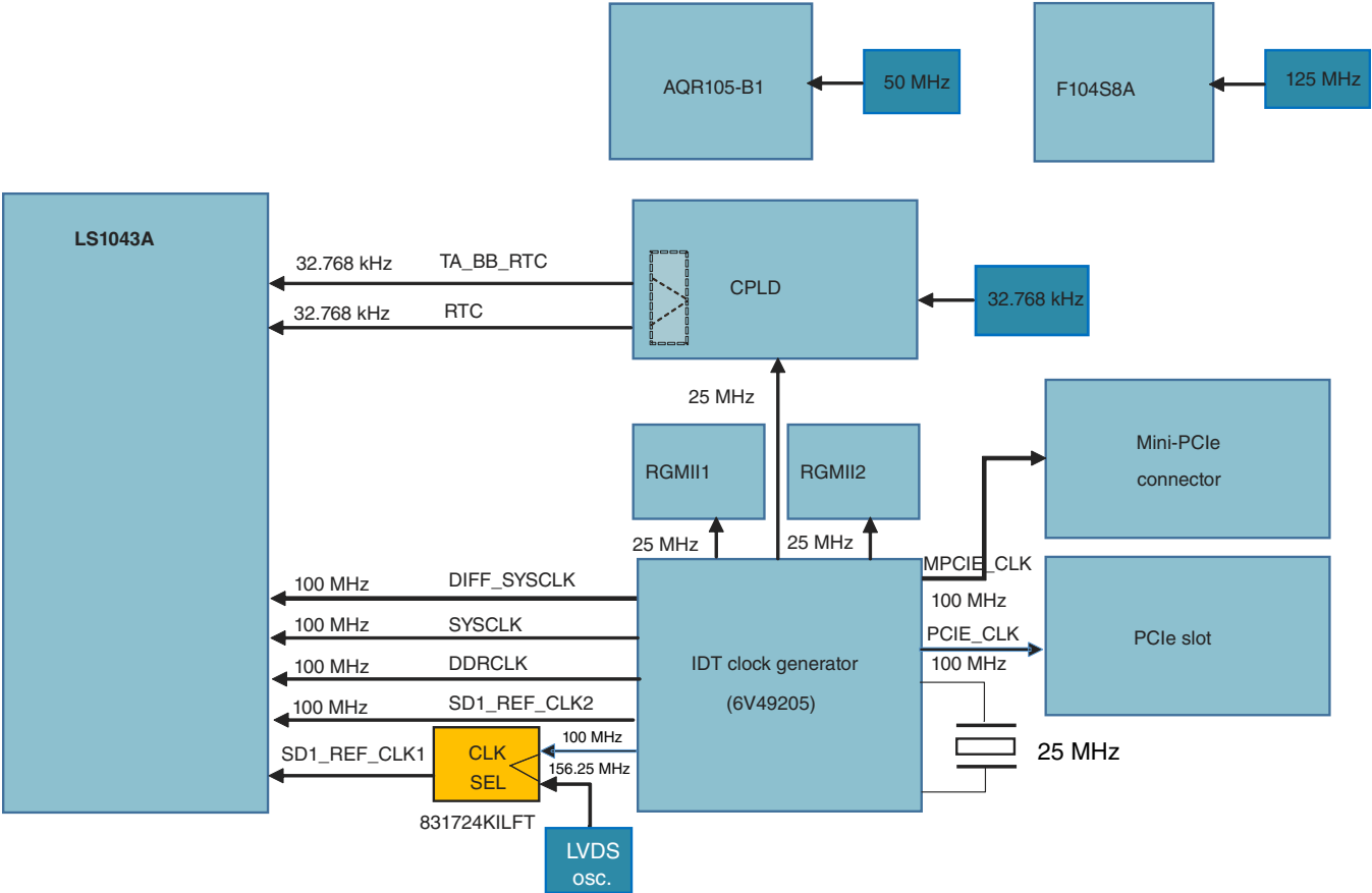
Figure 4-1. Clocking scheme
