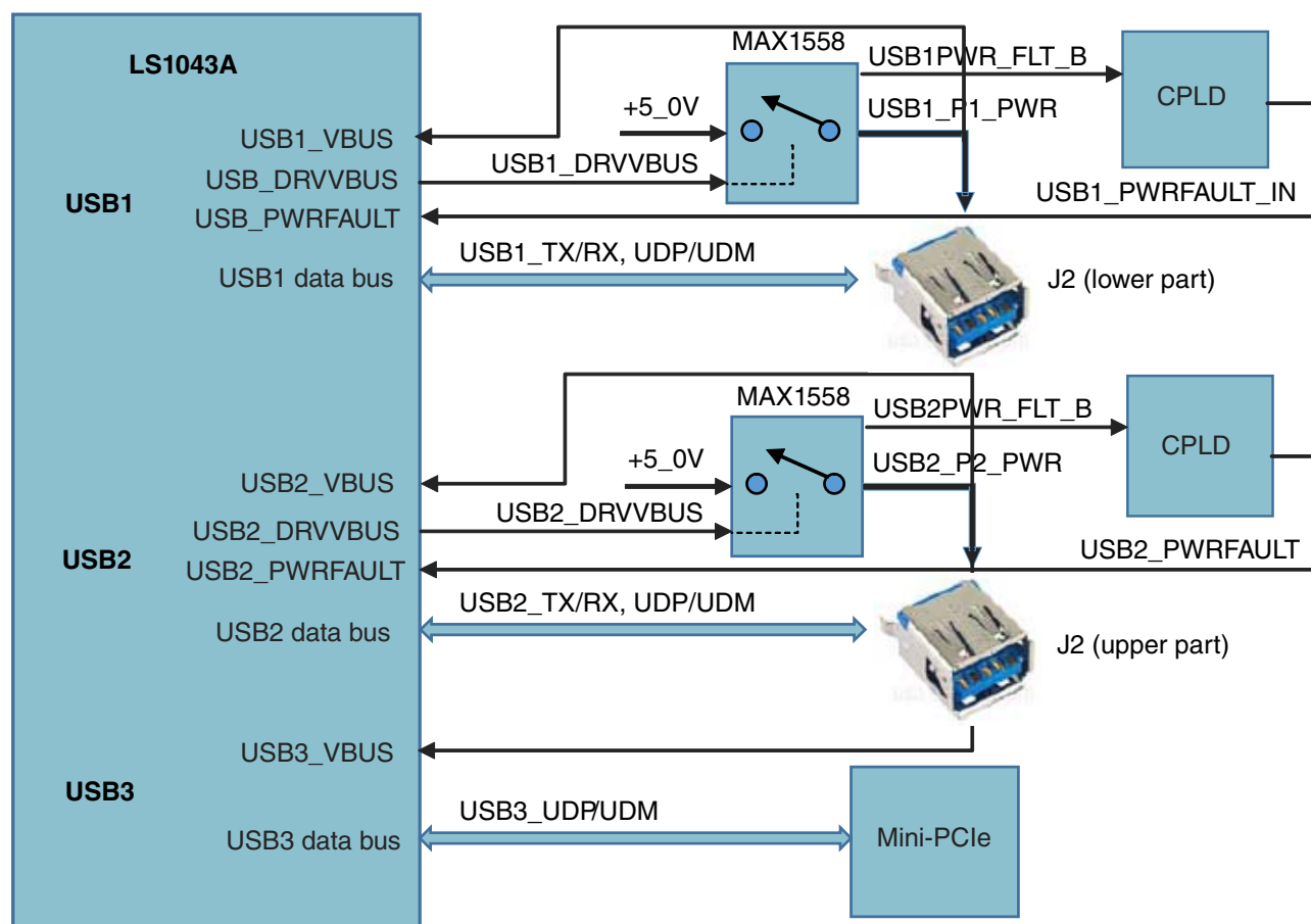
Figure 2-9. USB architecture
