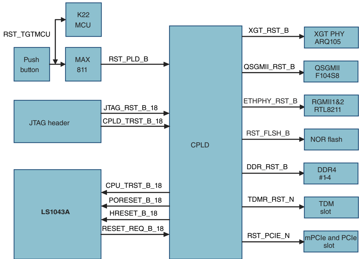
Figure 3-4. Reset architecture
