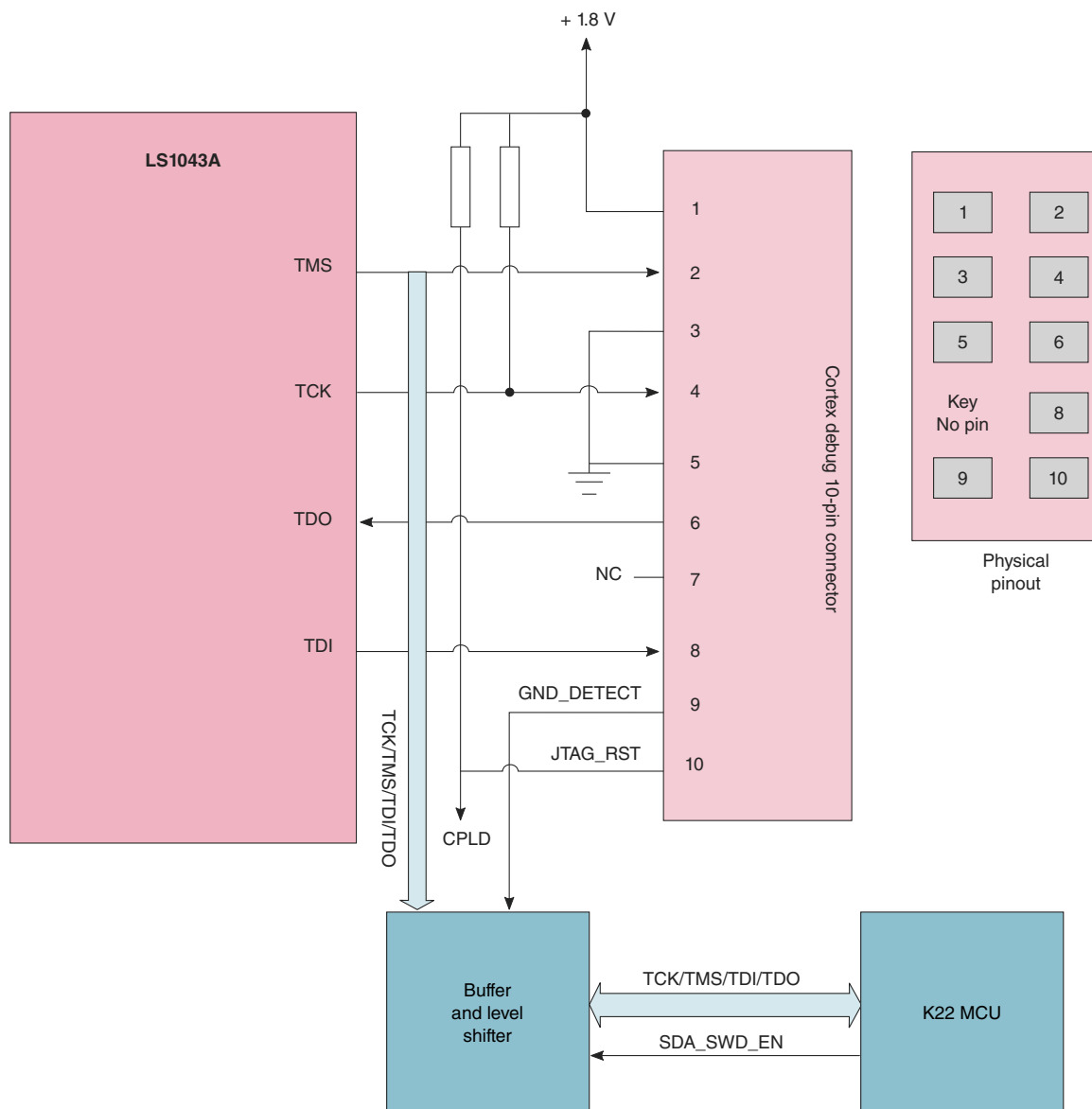
Figure 5-1. ARM/JTAG architecture
