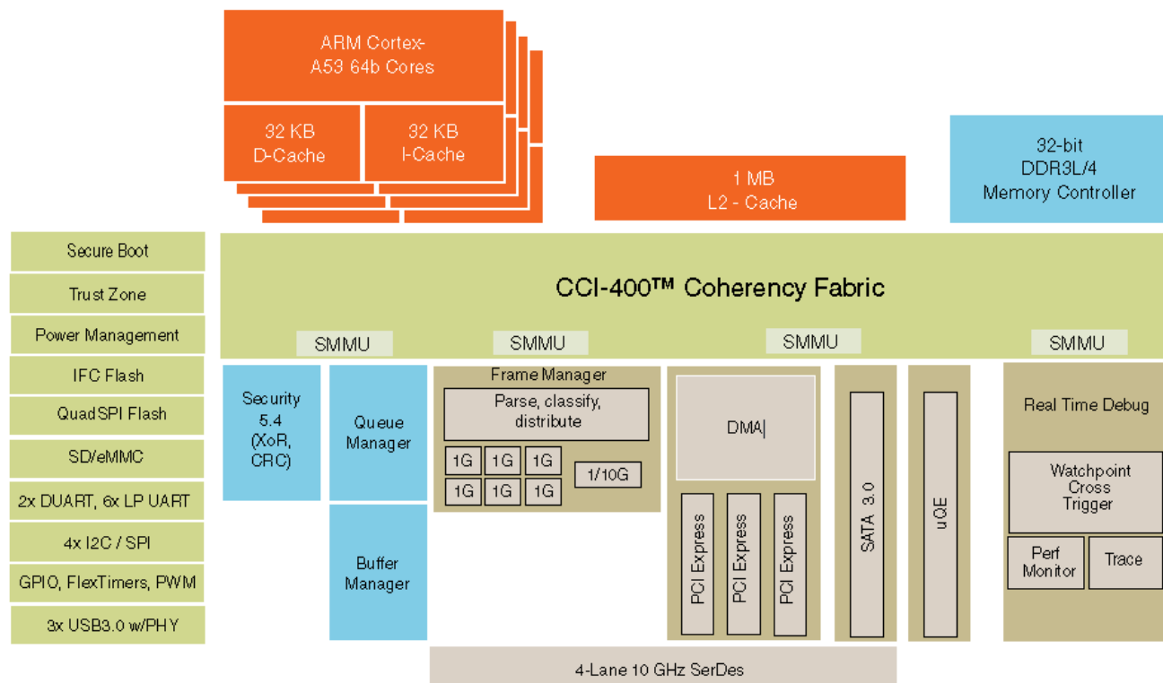
Figure 1-1. LS1043A processor block diagram
