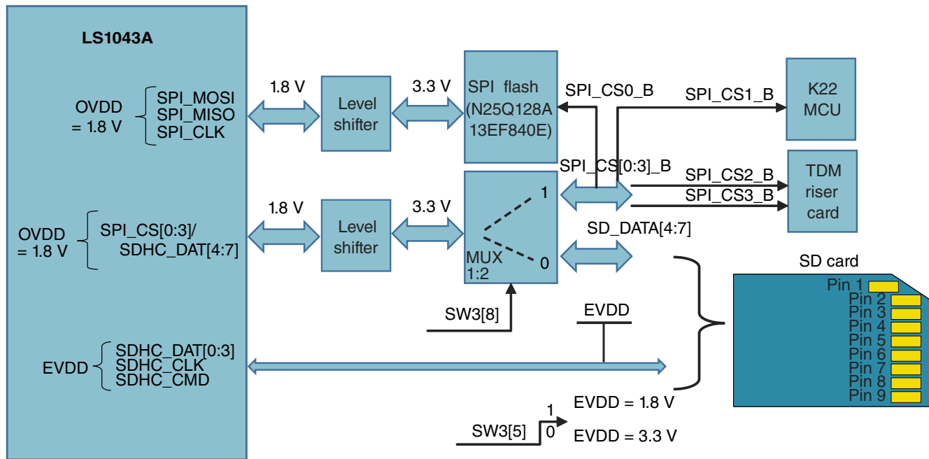
Figure 2-4. eSDHC connections
