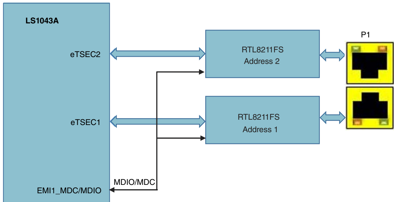
Figure 2-6. Ethernet interface
