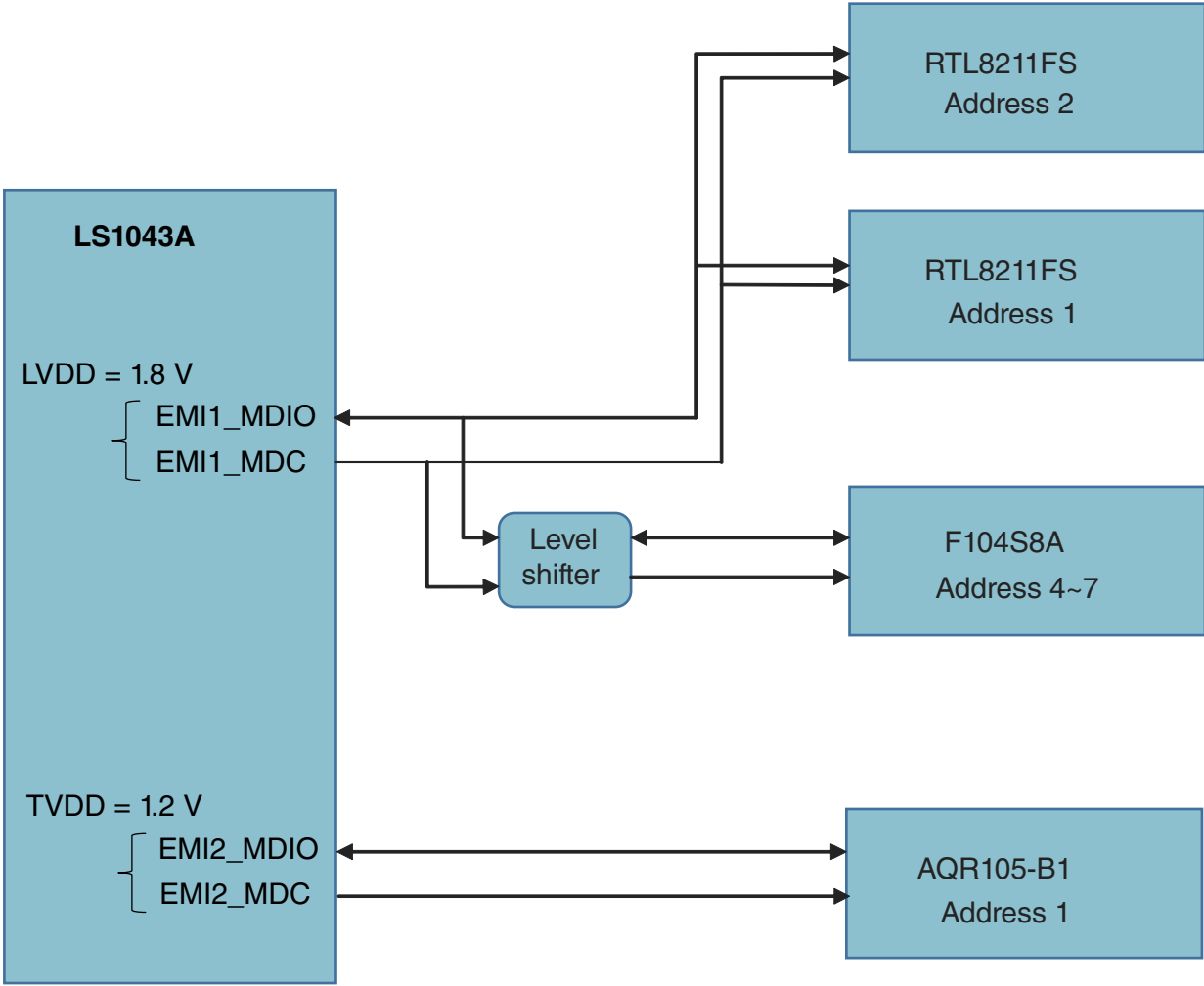
Figure 2-7. MII management buses
