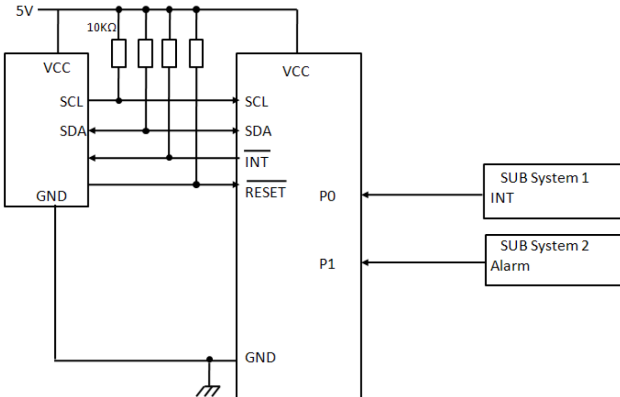
Figure 7: Typical application
