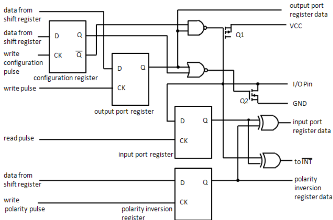
Figure 2: Simplified schematic of I/Os
