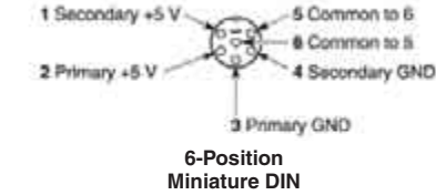
Contact ID Shown from Mating End of Station Connector
