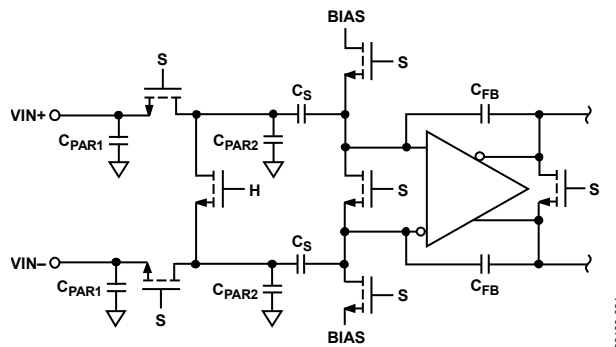
Figure 48. Switched-Capacitor Input
