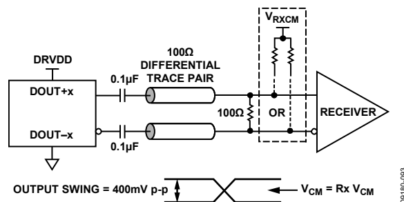
Figure 66. AC-Coupled Digital Output Termination Example
