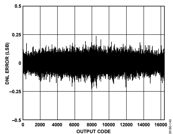
Figure 40. AD9644-155 DNL with f_{IN} = 30.3 MHz
