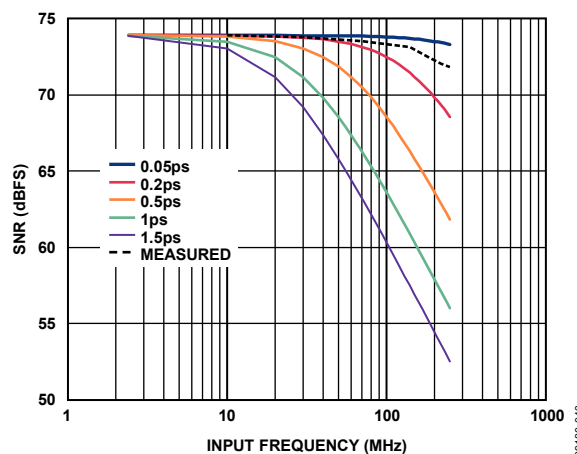
Figure 59. SNR vs. Input Frequency and Jitter
