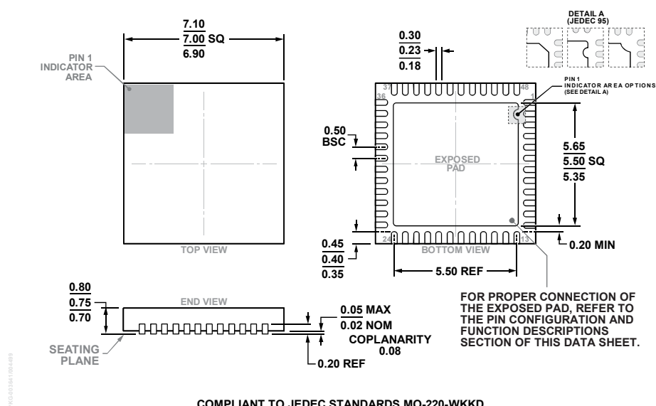
Figure 72. 48-Lead Lead Frame Chip Scale Package [LFCSP] 7 mm × 7 mm Body and 0.75 mm Package Height (CP-48-9)
