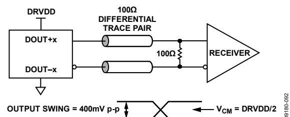
Figure 67. DC-Coupled Digital Output Termination Example
