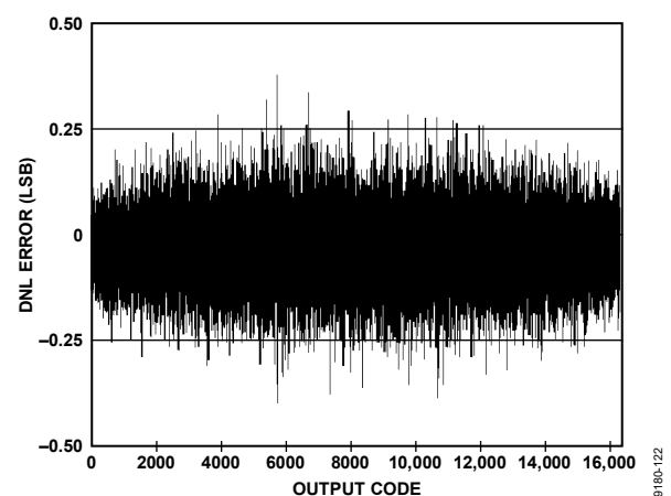
Figure 22. AD9644-80 DNL with f_{IN} = 30.3 MHz
