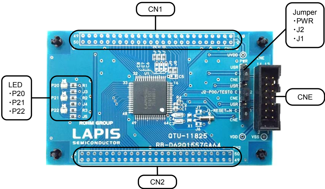
Fig. 1 ML62Q1557 Reference Board Outline Diagram
