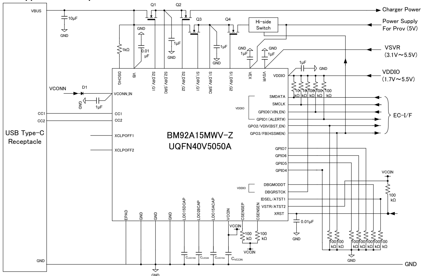
Figure 5-1 Application Example
