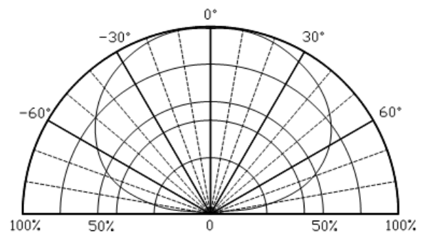
Directive Characteristics
