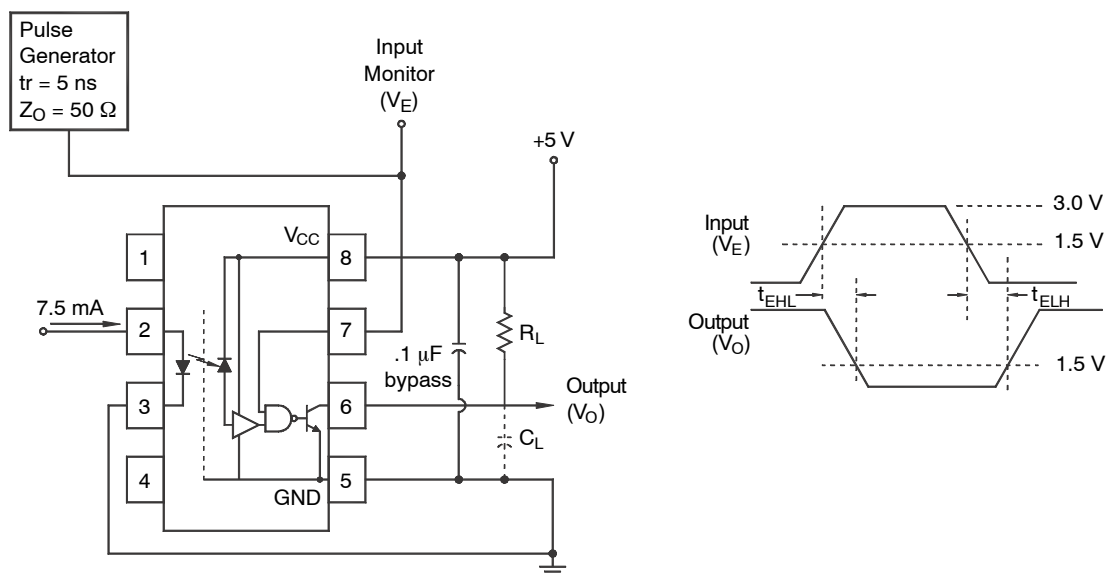
Figure 24. Test Circuit t_{EHL} and t_{ELH}
