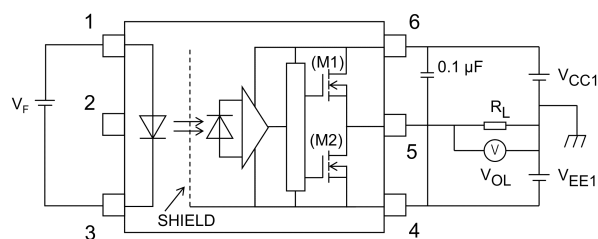
Fig. 13.1.4 V_{OL} Test Circuit
