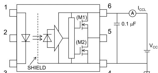
Fig. 13.1.6 I_{CCL} Test Circuit
