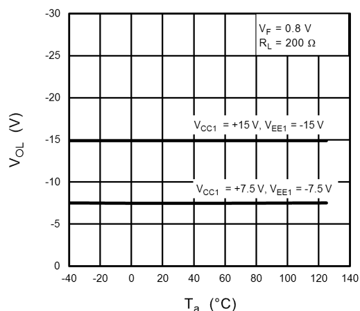
Fig. 13.2.7 V_{OL} - T_a
