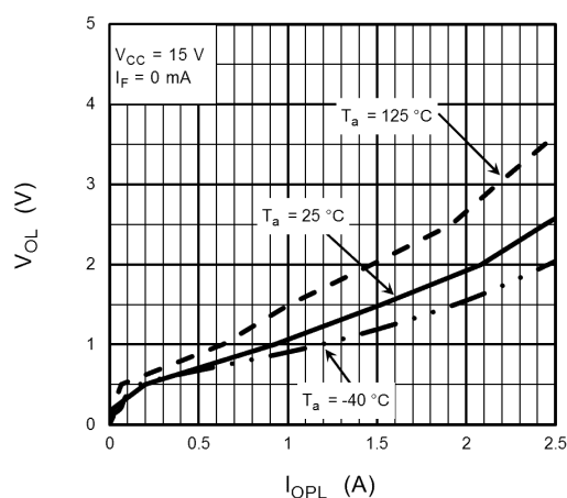
Fig. 13.2.9 V_{OL} - I_{OPL}
