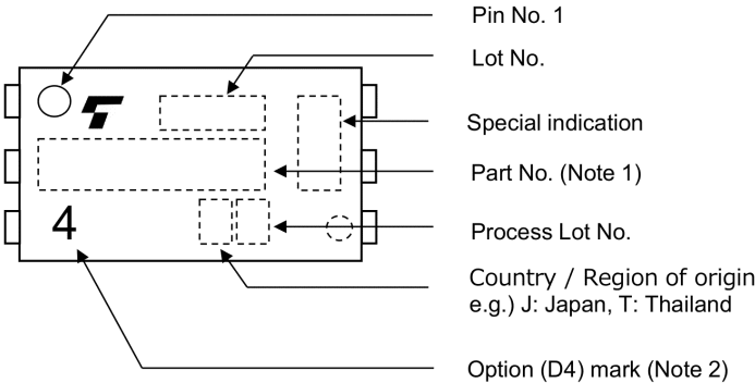
Fig. 17.4 Marking Example
