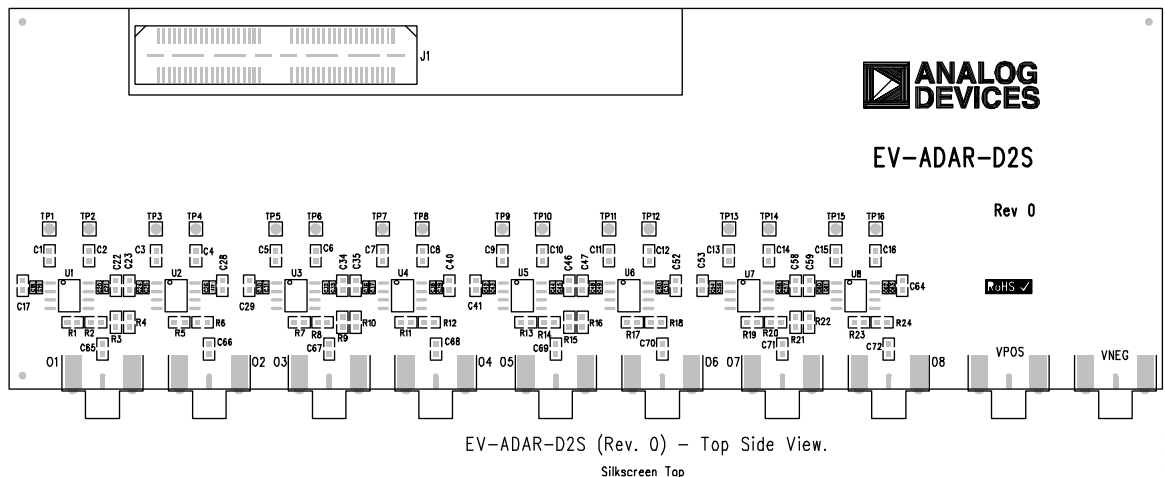
Figure 31. EV-ADAR-D2S Assembly
