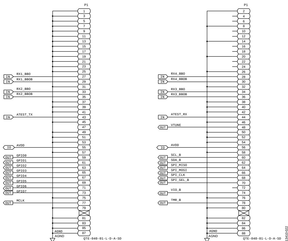
Figure 22. Evaluation Board Schematic (Page 13)
