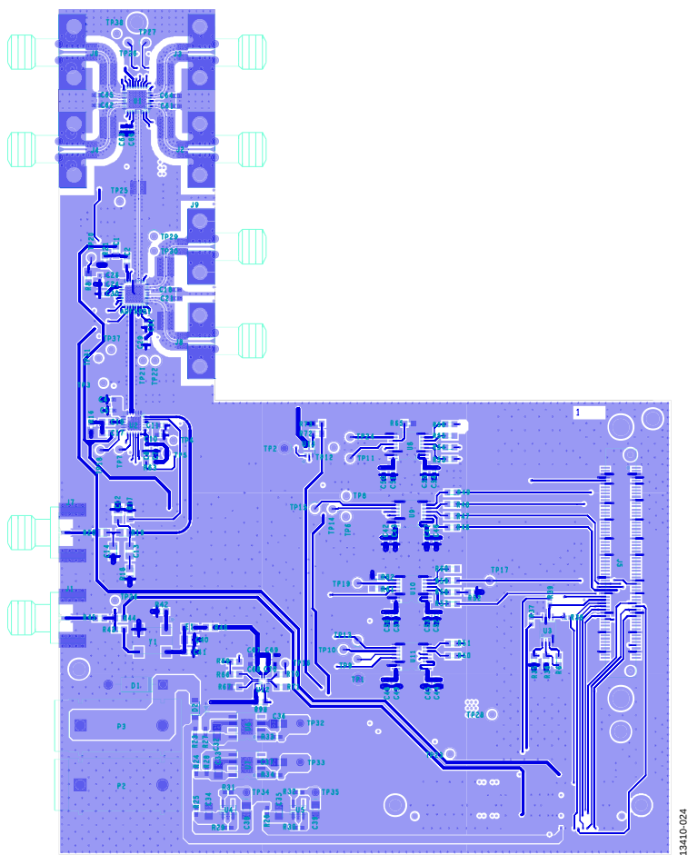
Figure 29. Layer 1 (Component Side)
