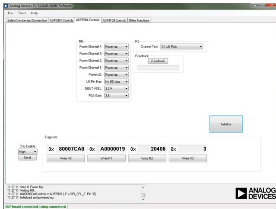
Figure 3. ADF5904 Controls
