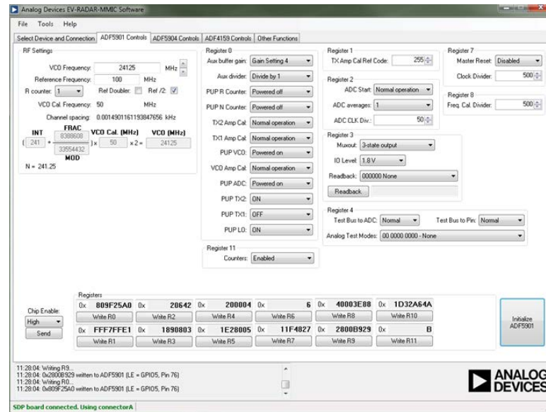
Figure 4. ADF5901 Controls
