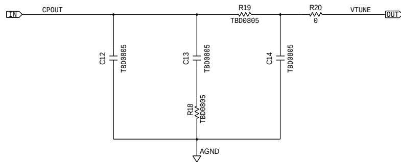
Figure 12. Evaluation Board Schematic (Page 3)
