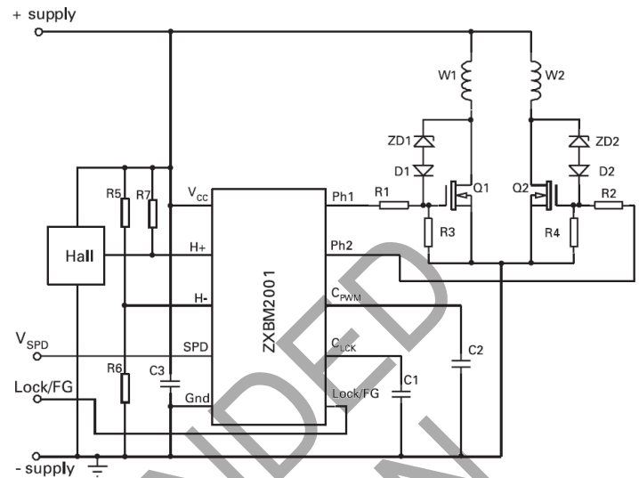
Figure 2 TYPICAL APPLICATION (ZXBM2001) using MOSFET power transistors
