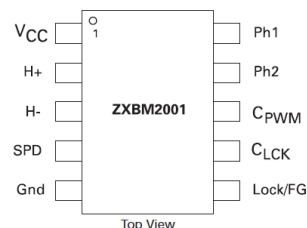
MSOP-10
