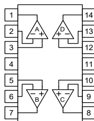
NJM2902M, NJM2902V NJM2902N (Discontinued)
