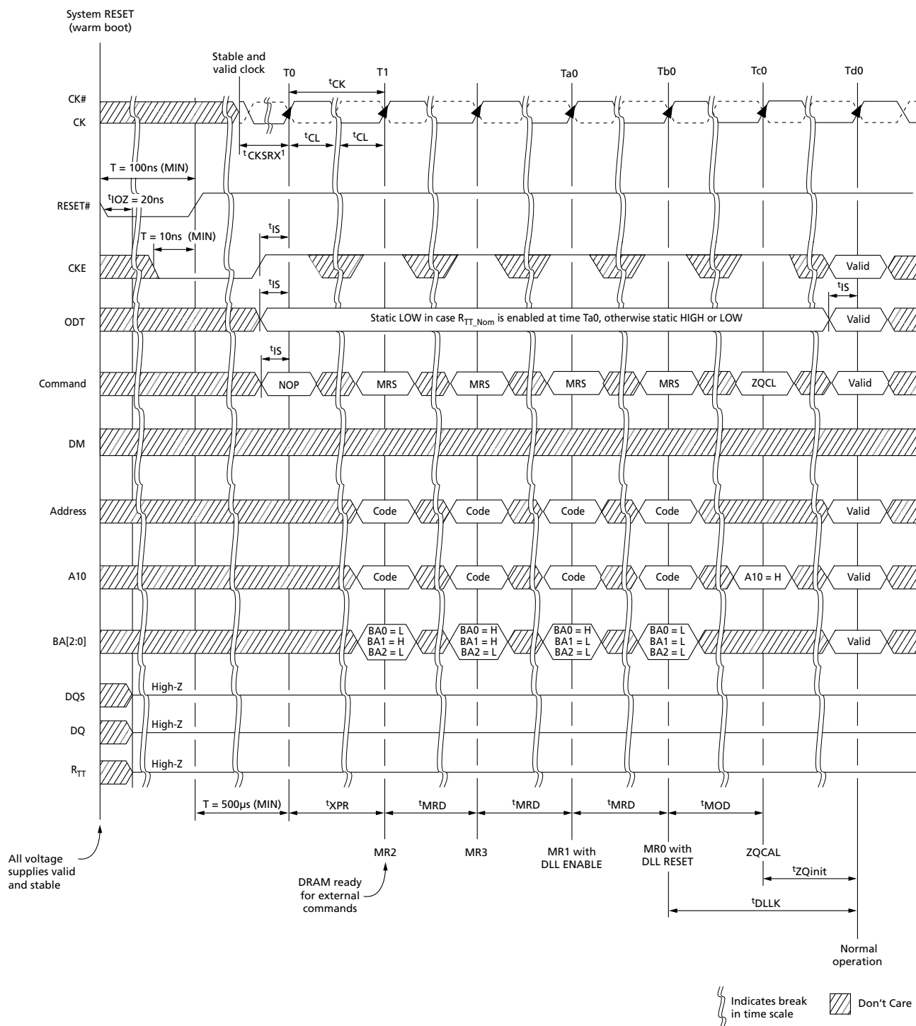
Figure 105: RESET Sequence
