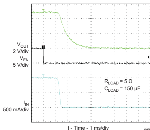
Figure 19. Turn-Off Response
