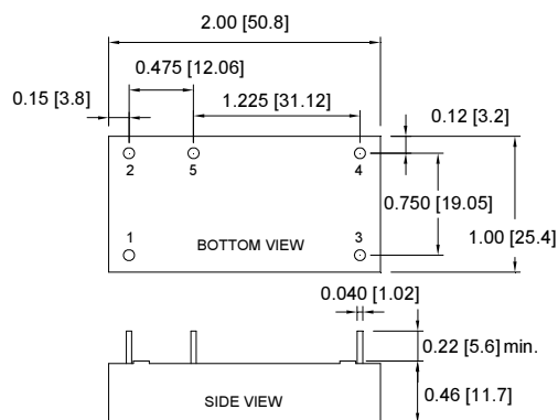
FM10-100 Package
