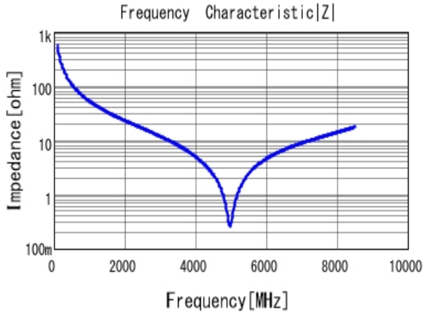
■ GCQ1555C1H2R9BB01 |Z| DC0V, 25degC
