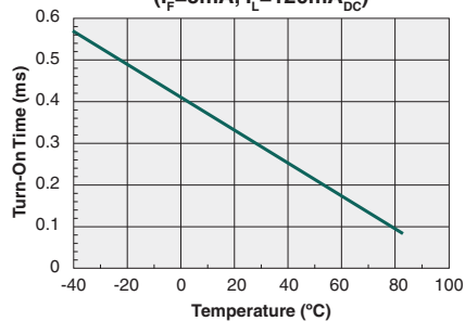
Typical Turn-On Time vs. Temperature ( I_F=5\text{mA} , I_L=120\text{mA}_{DC} )
