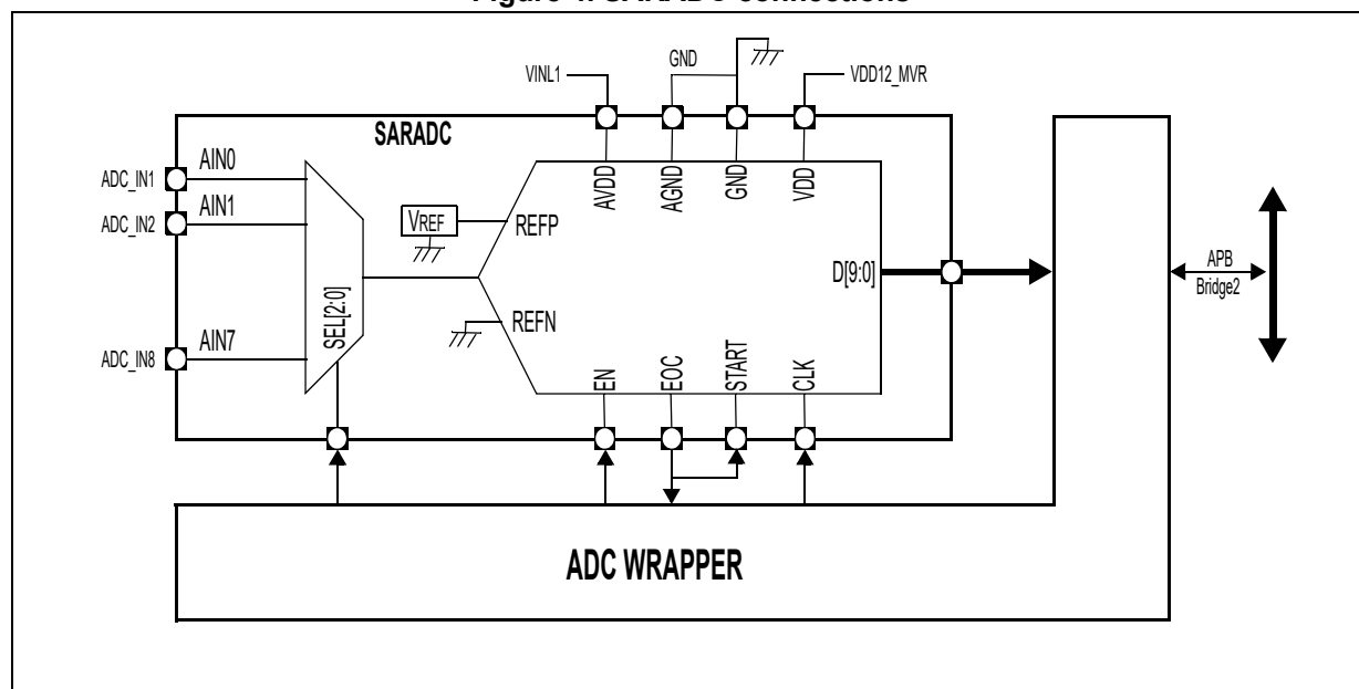
Figure 4. SARADC connections
