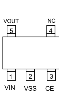
SOT-25 (TOP VIEW)
