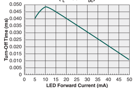
Typical Turn-Off Time vs. LED Forward Current ( I_L=250\text{mA}_{DC} )
