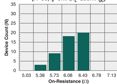
Typical On-Resistance Distribution (N=50, I_F=5\text{mA} , I_L=250\text{mA}_{DC} )
