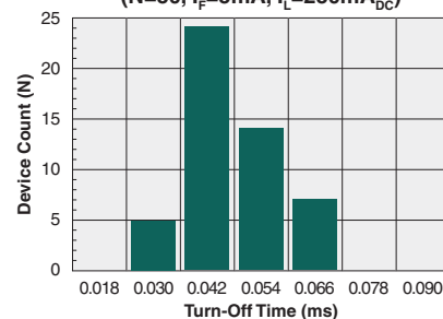
Typical Turn-Off Time (N=50, I_F=5\text{mA} , I_L=250\text{mA}_{DC} )
