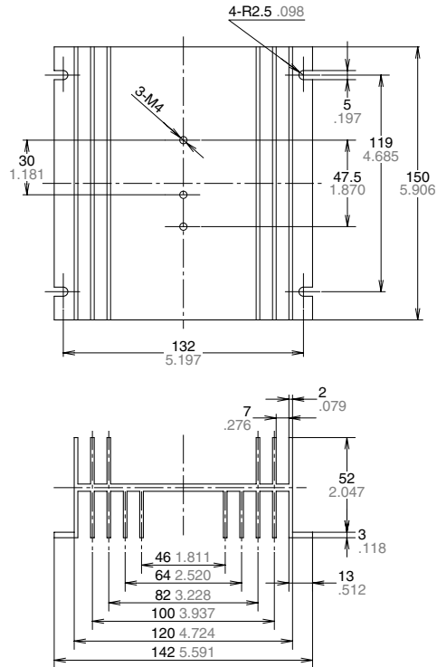
External dimensions
