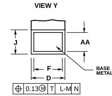
SECTION J1-J1 ROTATED 90° COUNTERCLOCKWISE
