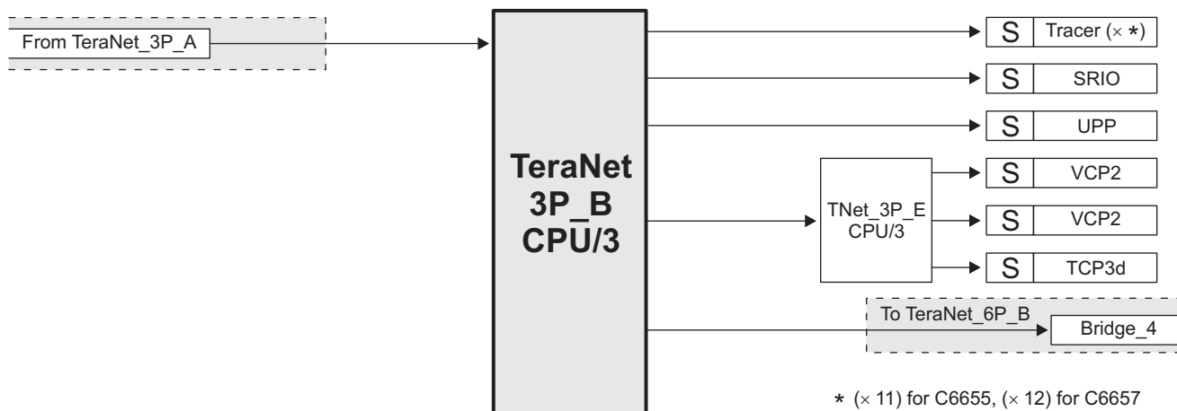
Figure 9-3. TeraNet 3P_B
