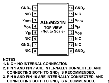
Figure 8. ADuM221N Pin Configuration
