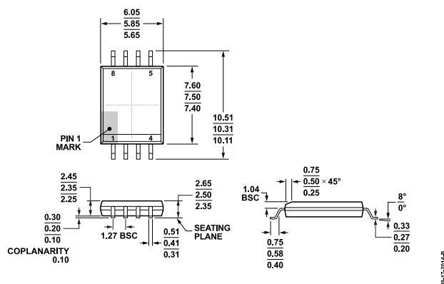
Figure 24. 8-Lead Standard Small Outline Package, with Increased Creepage [SOIC_IC]
