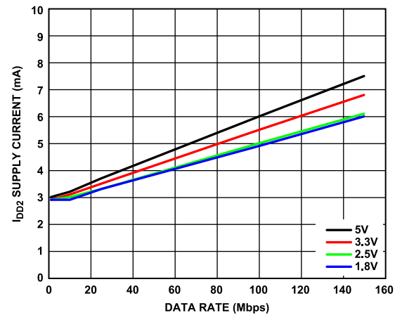
Figure 15. ADuM221N/ADuM226N I_{DD2} Supply Current vs. Data Rate at Various Voltages
