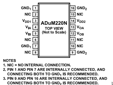
Figure 7. ADuM220N Pin Configuration
