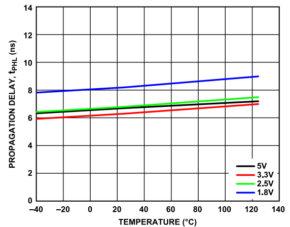
Figure 16. Propagation Delay for Logic Low Output ( t_{PHL} ) vs. Temperature at Various Voltages
