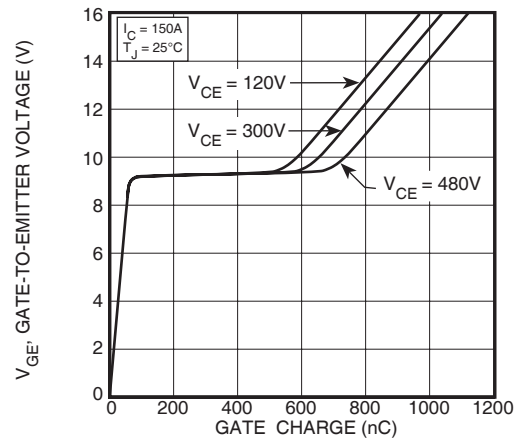
FIGURE 4, Gate Charge
