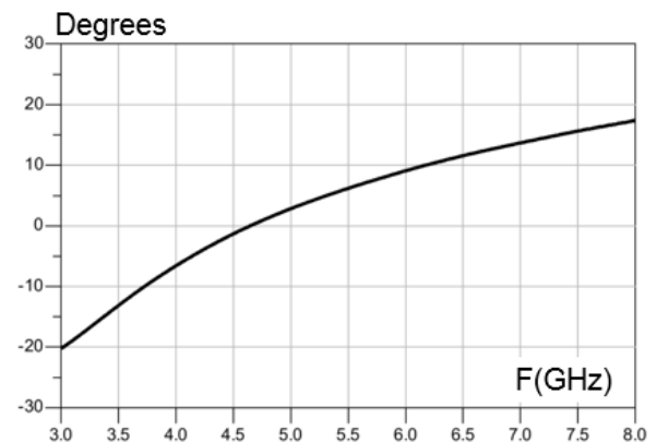
Figure 4. Phase balance (°)
