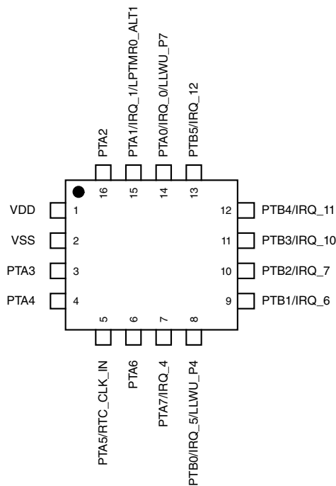
Figure 19. MCX C041 16-pin QFN pinout diagram
