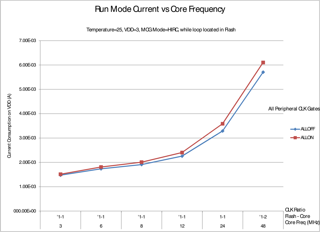
Figure 4. Run mode supply current vs. core frequency (loop located in flash)
