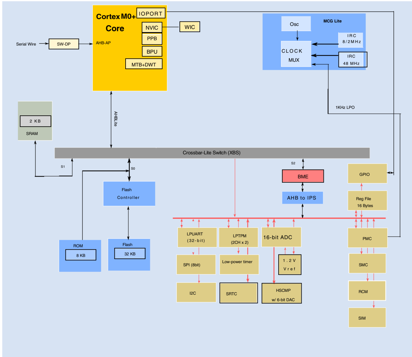
Figure 2. Architecture diagram
