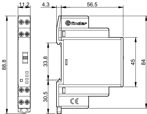
Type 19.91 Box clamp
