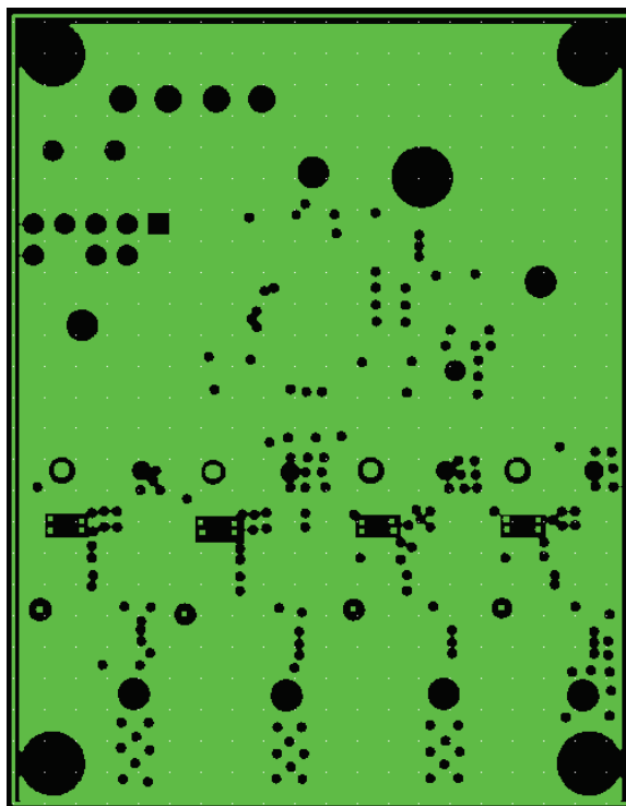
Figure 5: Ground Plane
