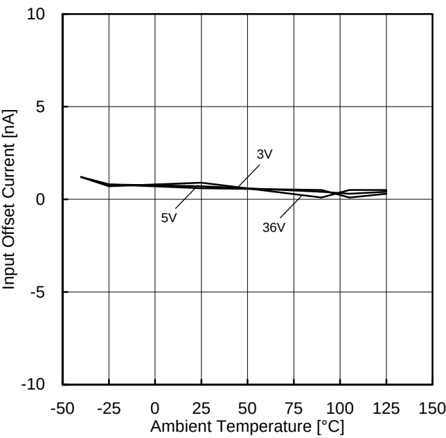
Figure 20. Input Offset Current vs Ambient Temperature (VICM=0V, EK=-1.4V)
