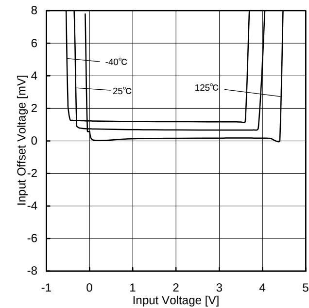
Figure 18. Input Offset Voltage vs Input Voltage (VCC=5V)
