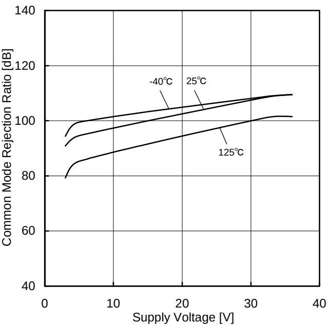
Figure 23. Common Mode Rejection Ratio vs Supply Voltage
