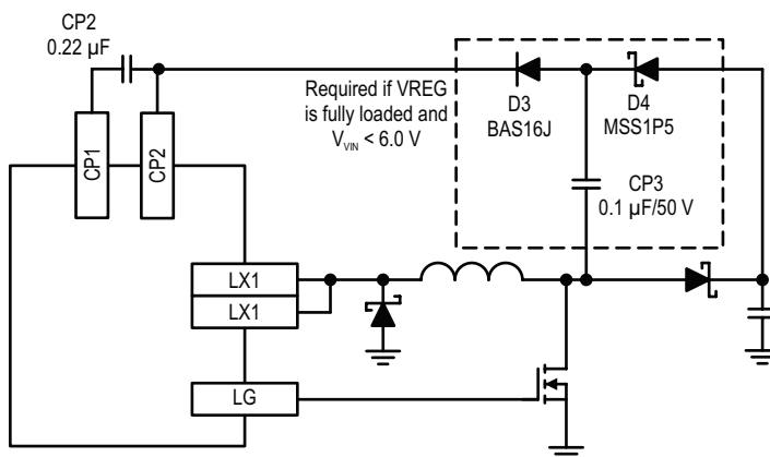
Figure 14: Charge pump enhancement components D3, D4, and CP3 are required if V_{VIN} < 6\ \text{V} .
