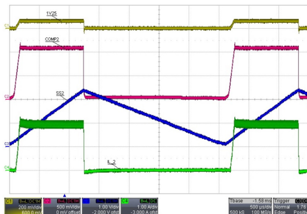
Figure 9: Synchronous Buck Hiccup Mode Operation when 1V25 is Shorted to GND and C_{SS2} = 10 nF
