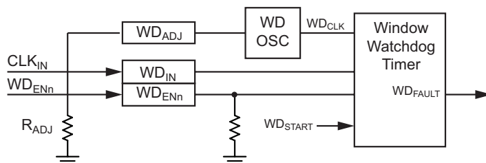
Figure 12: Watchdog Timer Block Diagram
