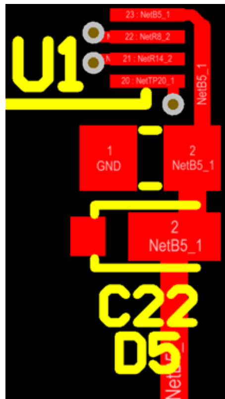
Figure 45: Recommended placement and routing of the LDO (V5P), output capacitor (C22), and negative clamp diode (D5).
