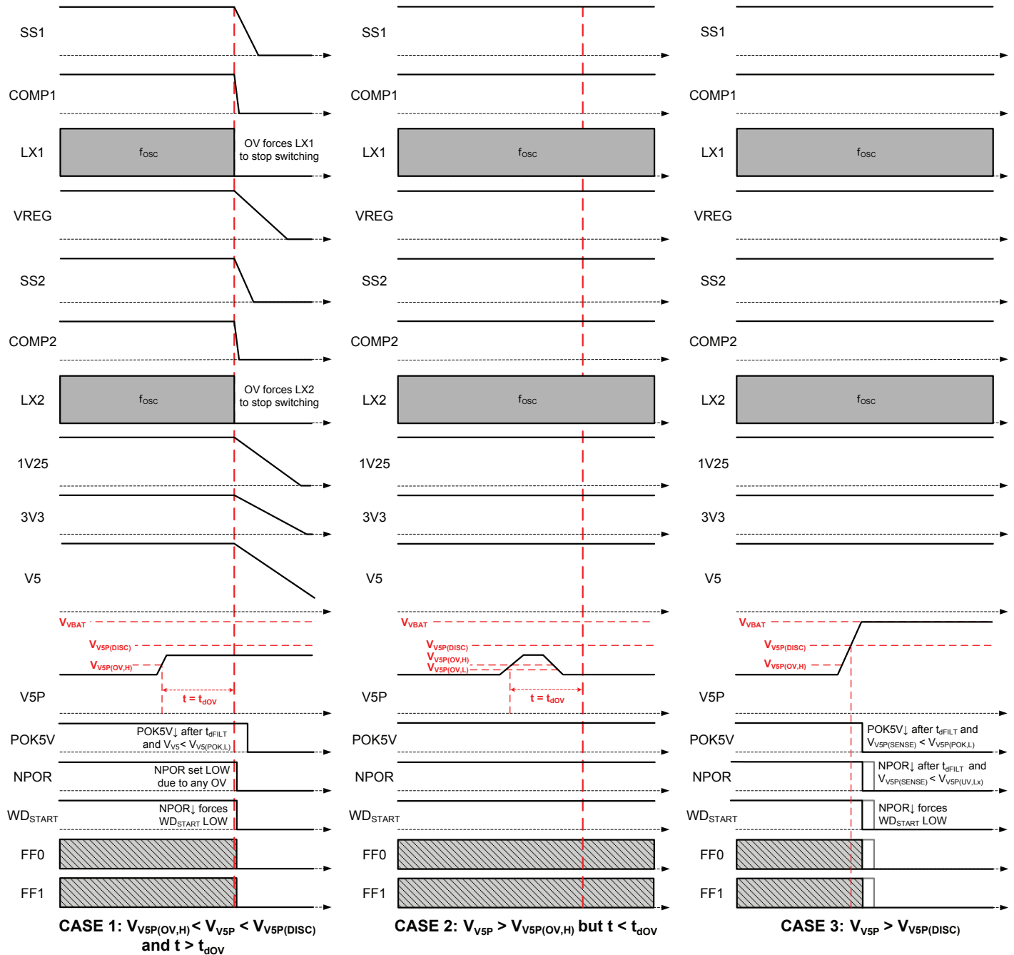
Figure 21: Possible Overvoltage Cases for V5P
