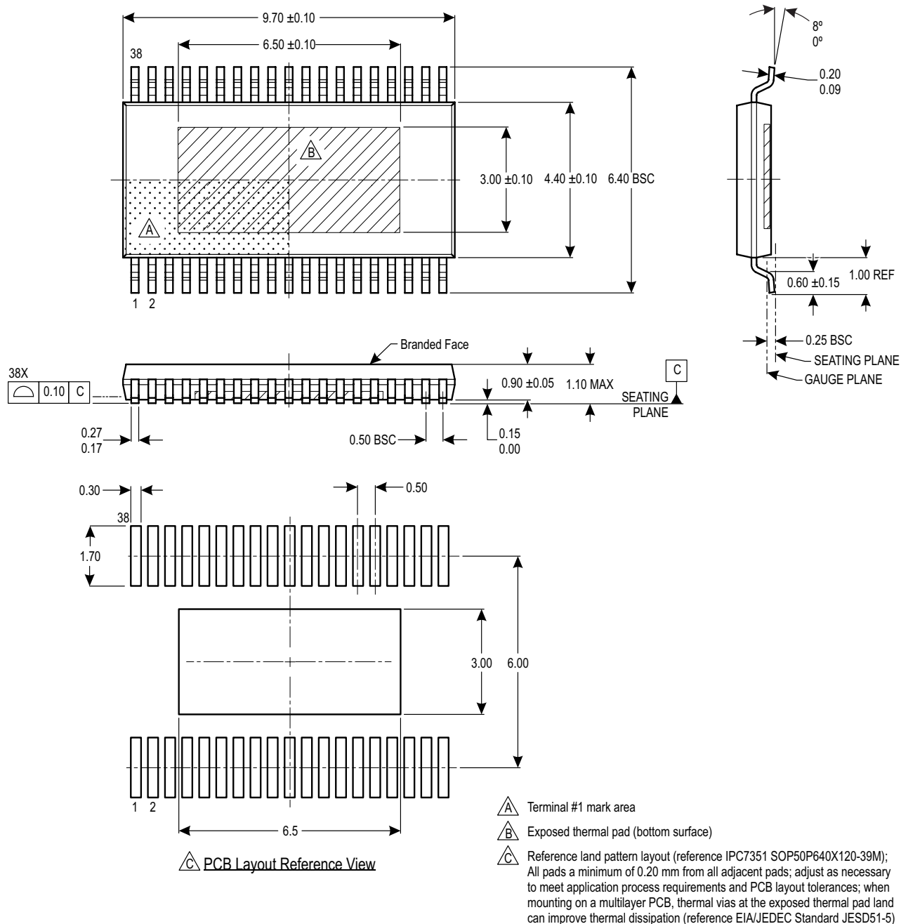
Figure 50: Package LV, 38-Pin eTSSOP
