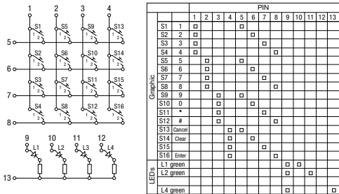
16 key piezo keypad with LED
