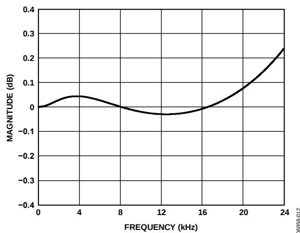
Figure 17. De-Emphasis Error, Audio Sampling Rate = 48 kHz
