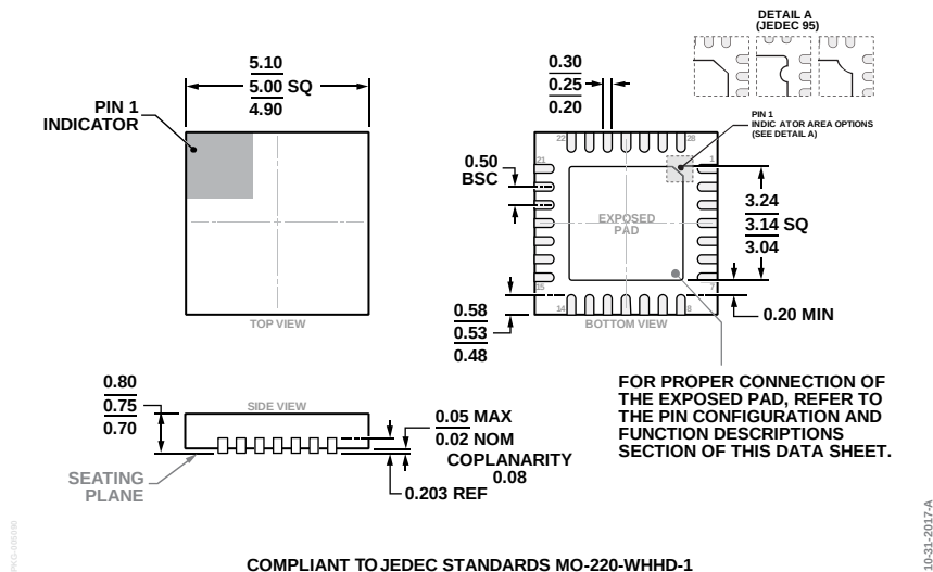
COMPLIANT TO JEDEC STANDARDS MO-220-WHHD-1 Figure 33. 28-Lead Lead Frame Chip Scale Package [LFCSP] 5 mm × 5 mm Body and 0.75 Package Height (CP-28-10) Dimensions shown in millimeters
