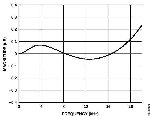
Figure 15. De-Emphasis Error, Audio Sampling Rate = 44.1 kHz
