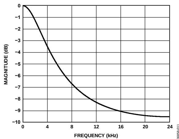
Figure 16. De-Emphasis Frequency Response, Audio Sampling Rate = 48 kHz
