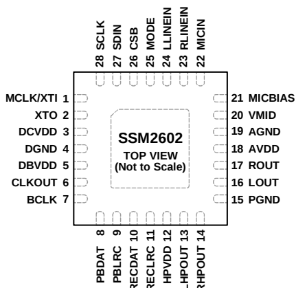
Figure 7. Pin Configuration
