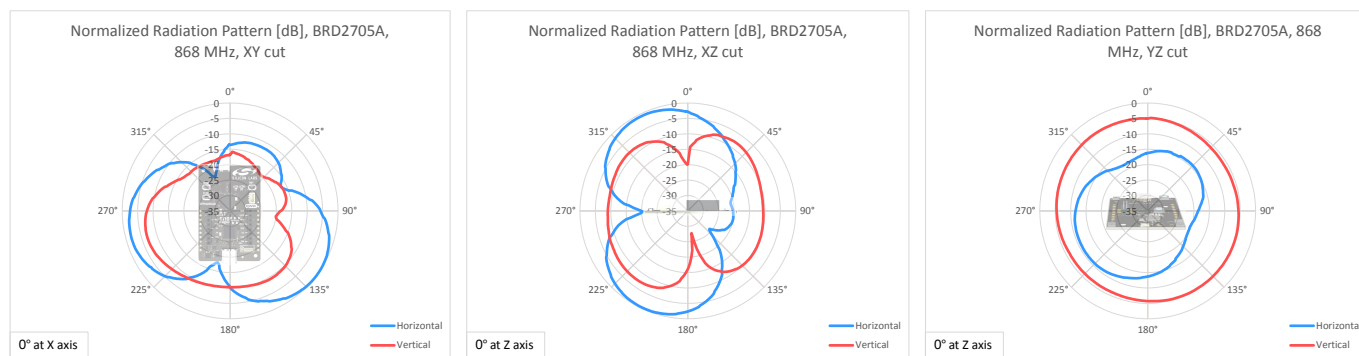
Figure 5.3. Antenna Pattern - 868 MHz
