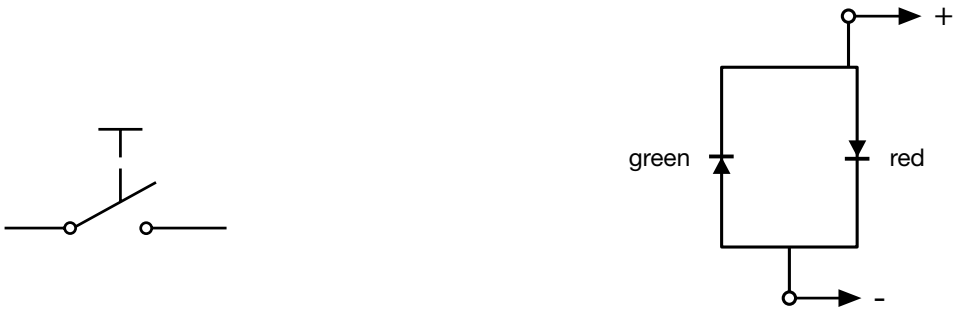
MCS 19 PI Bi-colour-LED
