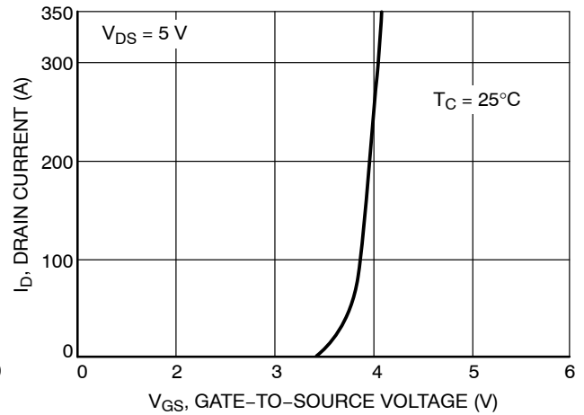
Figure 12. Transfer Characteristics
