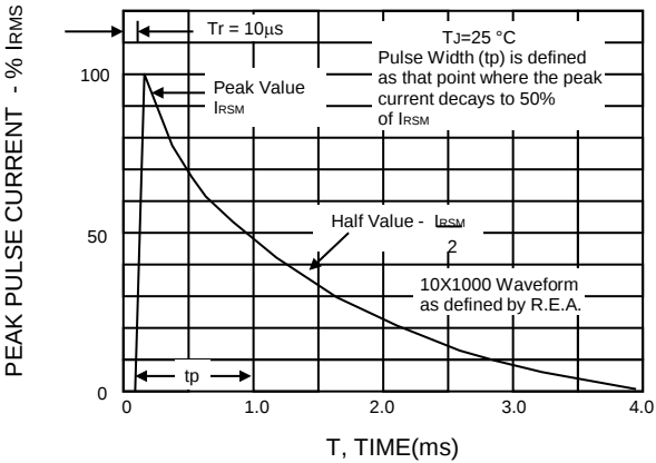
FIG.2 - PULSE WAVEFORM
