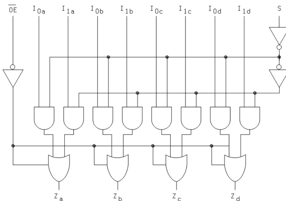
FIGURE 3. Logic diagram.
