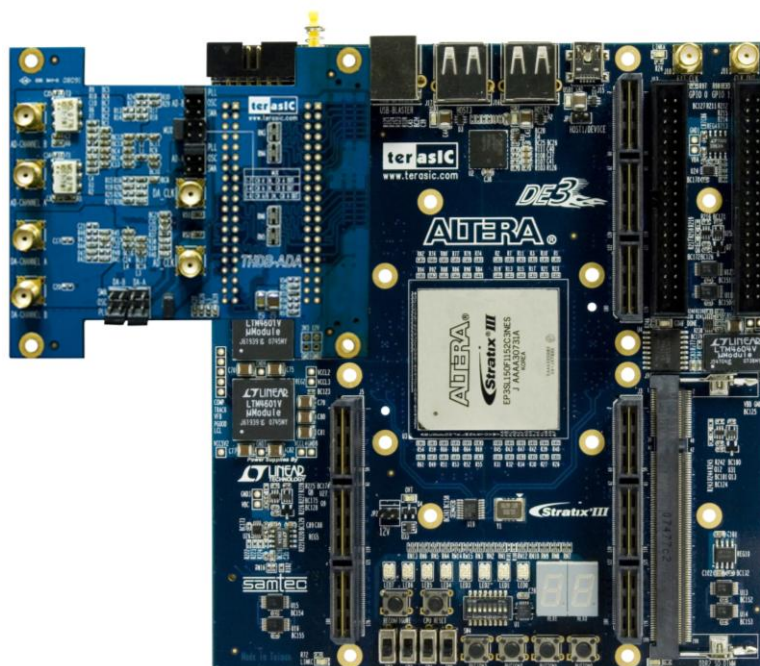
Figure 1-5 Connect ADA-HSMC with DE3 (HSTC connector D)
